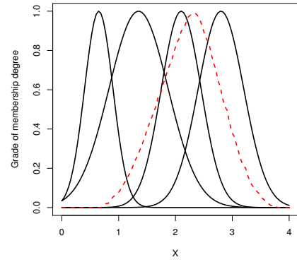
(a) FWA aggregation result
