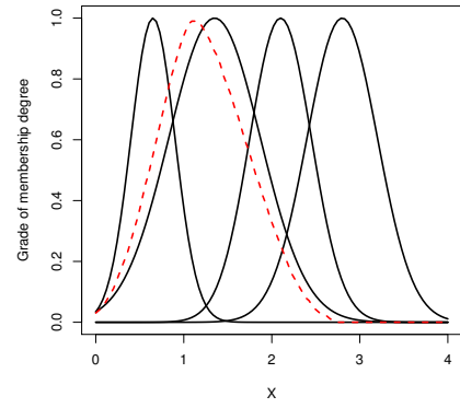
(b) Type-1 OWA aggregation result
