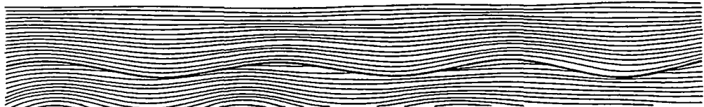
Scour-and-Drape Type
