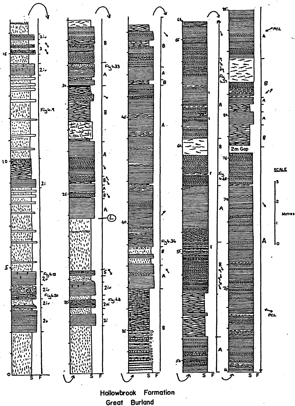
Text-fig. 1.3 Section from the Lynton Formation into the Hollowbrook Formation exposed at Great Burland.
