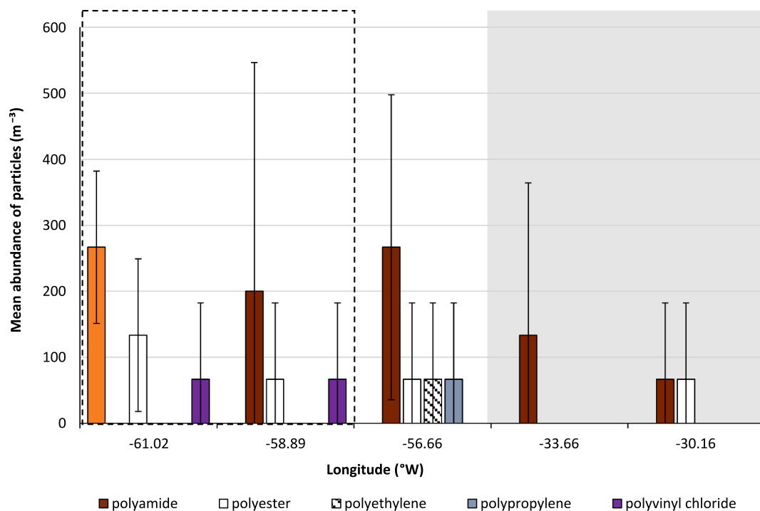
Fig. 4. The mean ( n = 3 ) abundance of synthetic particles \text{m}^{-3} of water sampled from a depth of -25 \text{ m} in the North Atlantic Ocean across the longitudinal transect. 'Inshore' sampling locations are depicted within the hatched boxes, the shaded region indicates sampling points from within the North Atlantic gyre and the remaining locations are 'open ocean'. Error bars show standard deviation.
