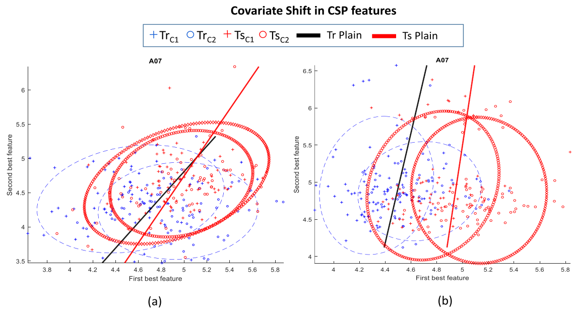
Fig. 1. Covariate shift (CS) between the training ( Tr ) and test ( Ts ) distributions of subject A07 in dataset-2A. (a) illustrates the CS in the \mu ( \mu ) band and (b) shows the CS in the \beta ( \beta ) band.
