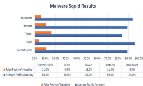
Fig. 6. Final test individual average accuracy for each malware type.
