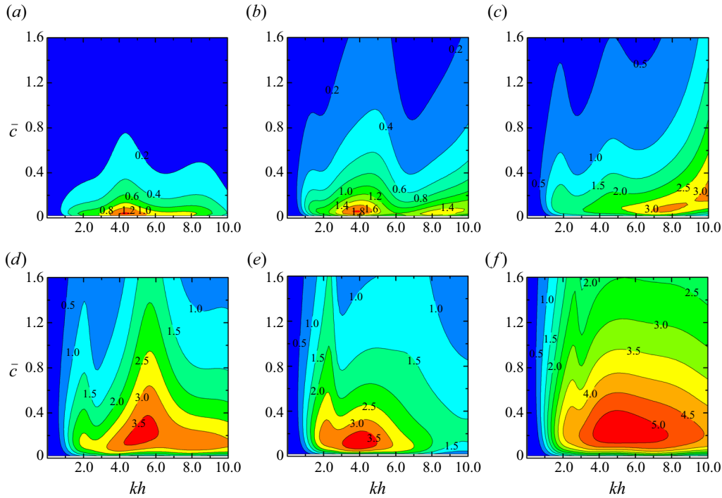
Figure 7. Contour plots for the variation of \eta_e as a function of wavenumber kh and PTO damping coefficient \bar{c} , for R/h = 2.0 , r_0/R = 0.5 and \beta = \pi/6 : (a) N = 1 , (b) N = 2 , (c) N = 3 , (d) N = 4 , (e) N = 5 , and (f) N = \infty .
