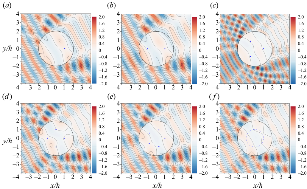
Figure 8. Deflection of the floating elastic disk, \text{Re}(\eta e^{-i\omega t})/A , and the near-field wave motion, \text{Re}(\eta_w e^{-i\omega t})/A , at t=0 for R/h=2.0 , r_0/R=0.5 and \beta=\pi/6 : (a) N=1 , (kh, \bar{c})=(4.28, 0.04) ; (b) N=2 , (kh, \bar{c})=(3.91, 0.06) ; (c) N=3 , (kh, \bar{c})=(7.64, 0.08) ; (d) N=4 , (kh, \bar{c})=(5.51, 0.20) ; (e) N=5 , (kh, \bar{c})=(4.65, 0.12) ; and (f) N=\infty , (kh, \bar{c})=(5.03, 0.24) .
