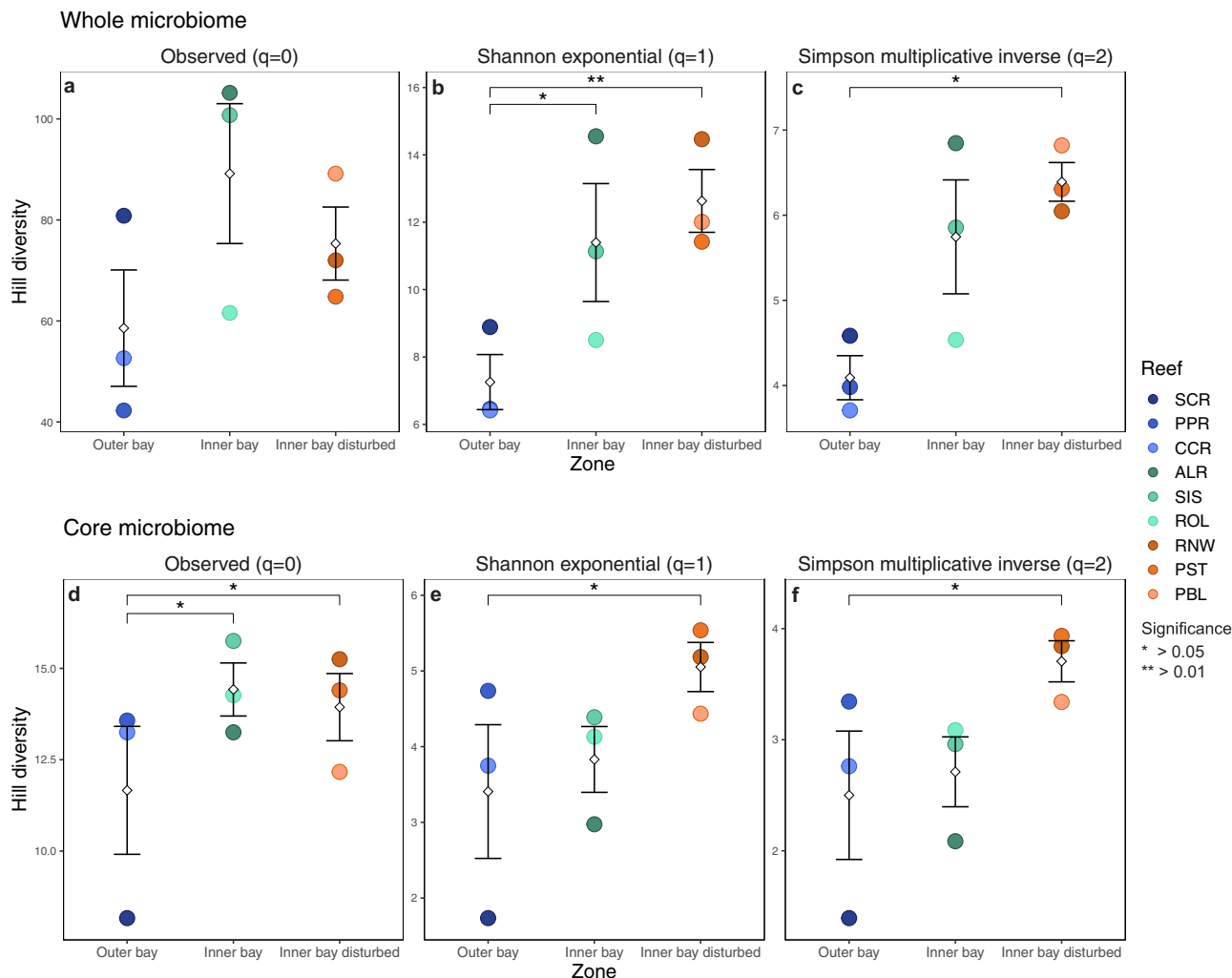
Fig. 3 Alpha diversity. Differences in diversity (mean ± SE) of ASVs between the whole gut microbiome (a–c) and the core gut microbiome (d–f) of Chaetodon capistratus across reefs. Alpha diversity was measured based on Hill numbers using three metrics that put more or less weight on common species. The observed richness (a, d) does not take into account relative abundances. Shannon exponential (b, e) weighs ASVs by their frequency. Simpson multiplicative inverse (c, f) overweighs abundant ASVs. Significance depicts differences in alpha diversity among reef zones (Kruskal–Wallis test with post hoc Dunn test). Diamonds depict means.
