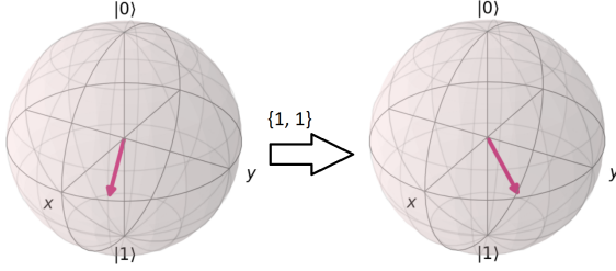
FIG. 3. A snapshot of rotating the qubit using the brain code \{1, 1\} .
