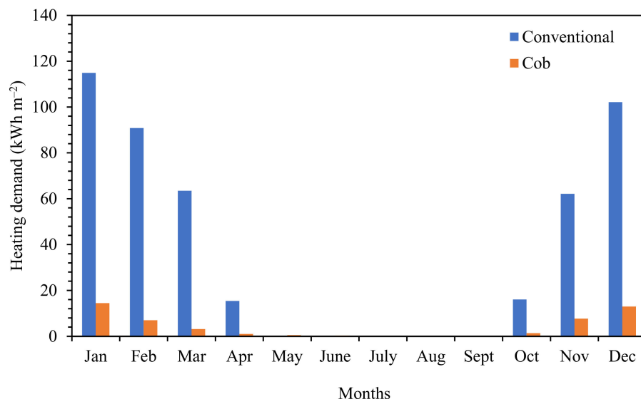
Figure 21. Heating demand for cob and conventional building over a year.
