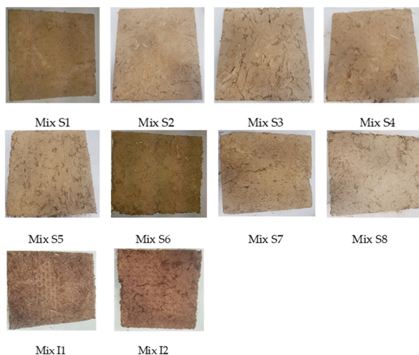
Figure 2. Photos of the studied structural and insulation cob samples.
