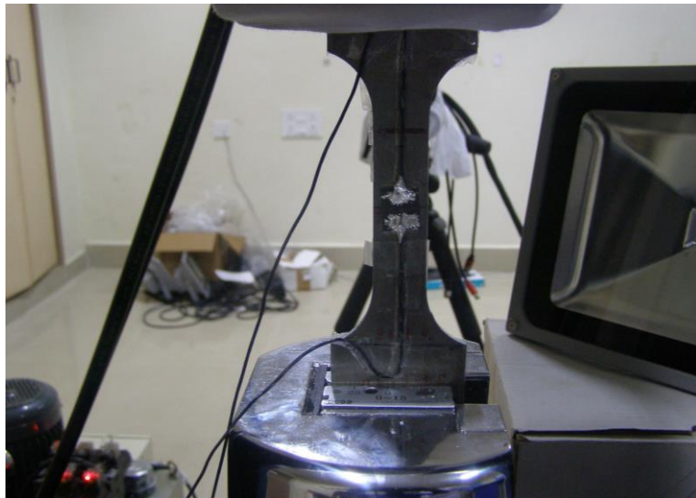
Figure 4: ASTM specimen with nano material based sensor attached at one side
