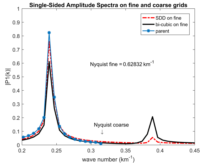
Figure 4. Amplitude spectra of parameter F on a zonal transect at y = 40 \text{ km} (see map in Fig. 1) based on data from the parent model on the coarse grid (blue-star line), SDD method (red) and bi-cubic interpolation (black). For clarity only the central part of the spectrum showing the peaks is presented.
