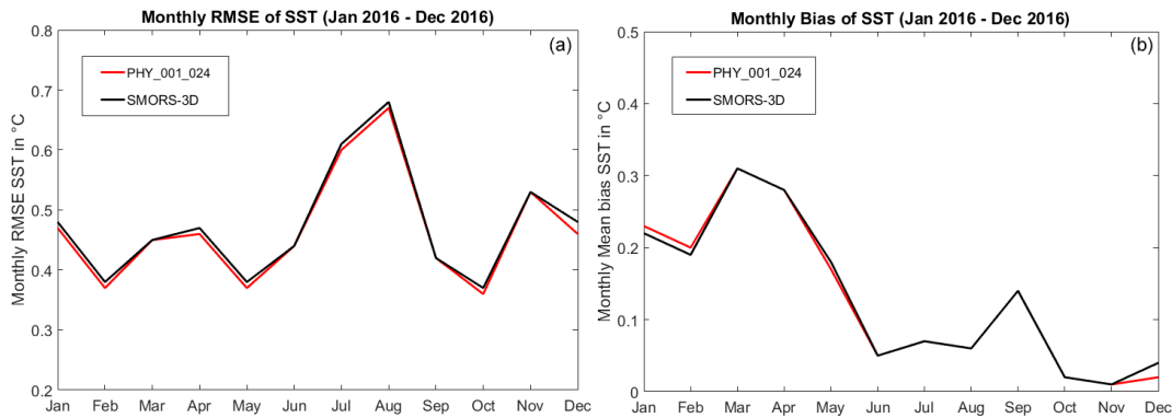
Figure 7. Monthly RMSE and bias comparisons: monthly RMSE (a) and monthly bias (b) between PHY_001_024 and OSTIA (red line) and between SMORS and OSTIA (black line).
