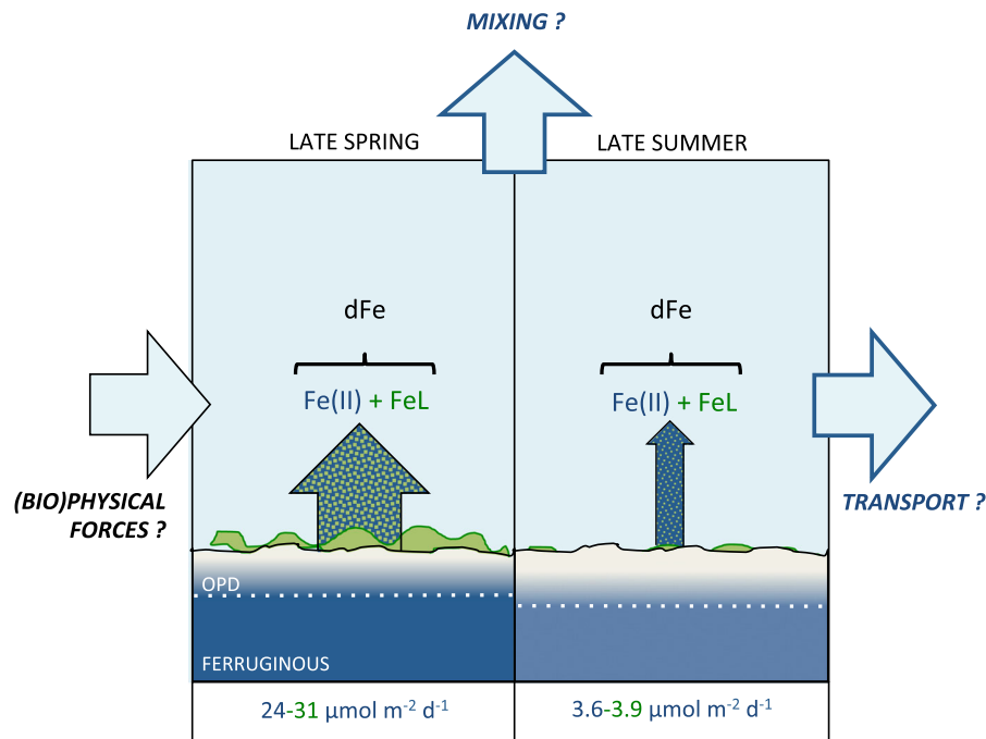
Fig. 10 Seasonal diffusive Fe(II) fluxes from the Celtic Sea Shelf and the proposed influence of stabilizing ligands. Calculated fluxes of Fe(II) to bottom water are indicated by arrow widths , and the potential influence of Fe(II)-stabilizing ligands by the density of green shading within arrows . Diffusive fluxes of Fe(II) which ignore the influence of ligands are smaller and correspond to minimum flux values described for each season. A shoaling of the oxygen penetration depth (OPD), increase in the surface porewater inventory of dFe(II) and an increase in the diffusive flux of dFe(II) to bottom waters coincides with the enhanced supply and decomposition of phytodetritus at the seafloor in late spring. An apparent 10–20 fold reduction in Fe(II) oxidation rates over empirical
