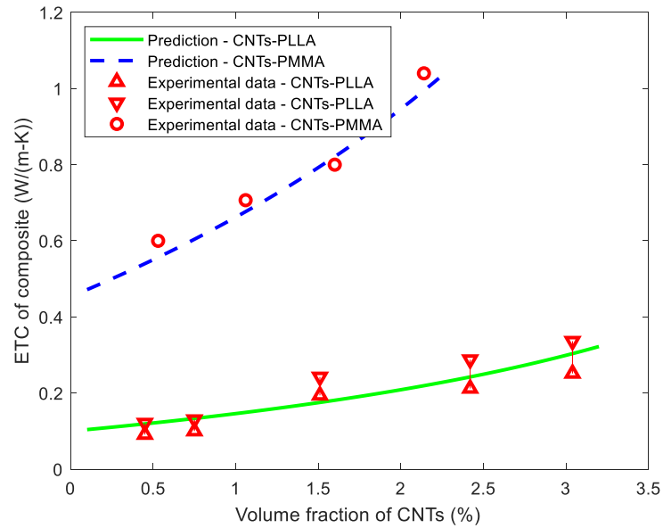
Fig.7 Comparison between analytically predicted and experimentally measured ETCs of CNTs-reinforced polymer composites ( k_2=0.10 \text{ W}/(\text{m}\cdot\text{K}) , \lambda=8 , hR_1=5k_2 for PLLA and k_2=0.45 \text{ W}/(\text{m}\cdot\text{K}) , \lambda=8 , hR_1=5k_2 for PMMA).
