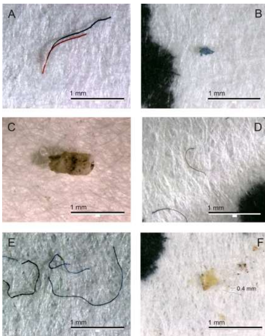
183 Figure 2. Microplastic particles found in juvenile fish of four fish species sampled from four mangroves in KwaZulu-Natal, South Africa. A: 184 particles of rayon (red and blue), B: blue fragment of PVC, C: opaque fragment of PVC from Durban Harbour mullet, D: polyester fibre, E: rayon 185 fibres and F: polyethylene fragment from a thornfish in Umgeni.
