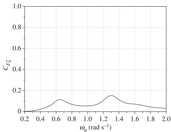
Figure 7. Behaviour of the capture width ratio in random seas C_{F\zeta} of the array versus peak frequency \omega_p . The PTO-coefficient \nu_{PT0} = 10^4 \text{ kg m}^2 \text{ s}^{-1} is optimized for the out-of-phase eigenfrequencies.
