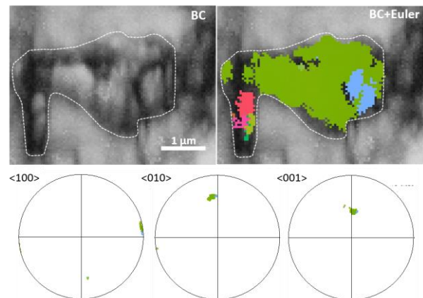
Figure 1: EBSD Band contrast (BC) and Euler maps of baddeleyite within lowest shock NWA 4480. Pole figures show baddeleyite hosts simple, magmatic twinning.
