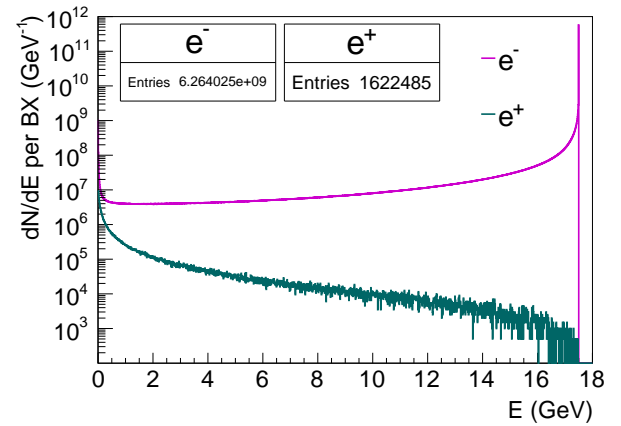
Figure 20. Energy spectra of electrons and positrons observed in the simulation with a tungsten target of 35 \mu\text{m} ( 1\%X_0 ) thickness for one bunch crossing. The electron spectrum also includes electrons from the beam which did not interact with the converter.
