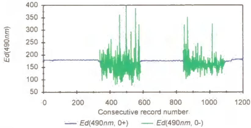
Fig 5.5. Ed(490) data collected above and below the air sea interface. The above surface measurements were adjusted for the immersion coefficient, which for the PRR-600 at 490nm , is Ed(0) = 0.796 \cdot Ed(0^+) . The units of irradiance are \mu W cm^{-2} nm^{-1} .
