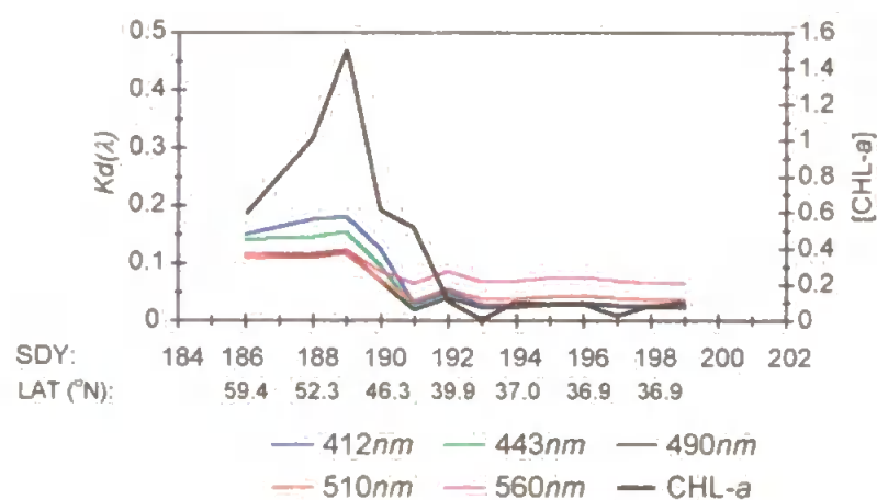
Figure 7.6. (a) Rrs(\lambda, 0') against time (SDY) and the corresponding latitudinal position of the sampling site and (b) the corresponding Kd(\lambda) values derived from analyses of radiometric profiles carried out during the PRIME study. The units for Rrs(\lambda) are sr^{-1} ; Kd(\lambda) : m^{-1} , and mg\ m^{-3} for Chlorophyll-a (CHL-a).
