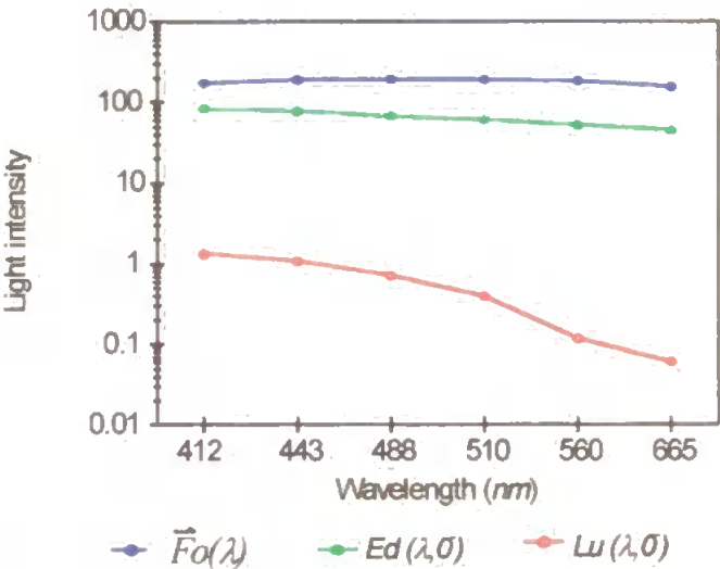
Figure 2.9 Values over the SeaWiFS bands for Lu(\lambda,0^+) derived from profile measurements. Also displayed are corresponding Ed(\lambda,0^+) data and \bar{F}_0(\lambda) (the extraterrestrial solar constant). The units for Ed(\lambda,z) and \bar{F}_0(\lambda) are \mu W\ cm^{-2}\ nm^{-1} and for Lu(\lambda,z) and are \mu W\ cm^{-1}\ nm^{-2}\ sr^{-1} .
