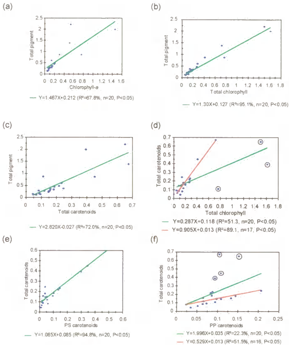
Figure 7.10 Regression analyses of the key pigments derived from the AMT-1 study: (a) chlorophyll-a to total pigments, (b) total chlorophyll to total pigment, (c) total carotenoids to total pigment, (d) total carotenoids to total chlorophyll, (e) photosynthetic carotenoids to total carotenoids, (f) photoprotective carotenoids to total carotenoids. The units for concentration of all pigments are mg\ m^{-3} .
