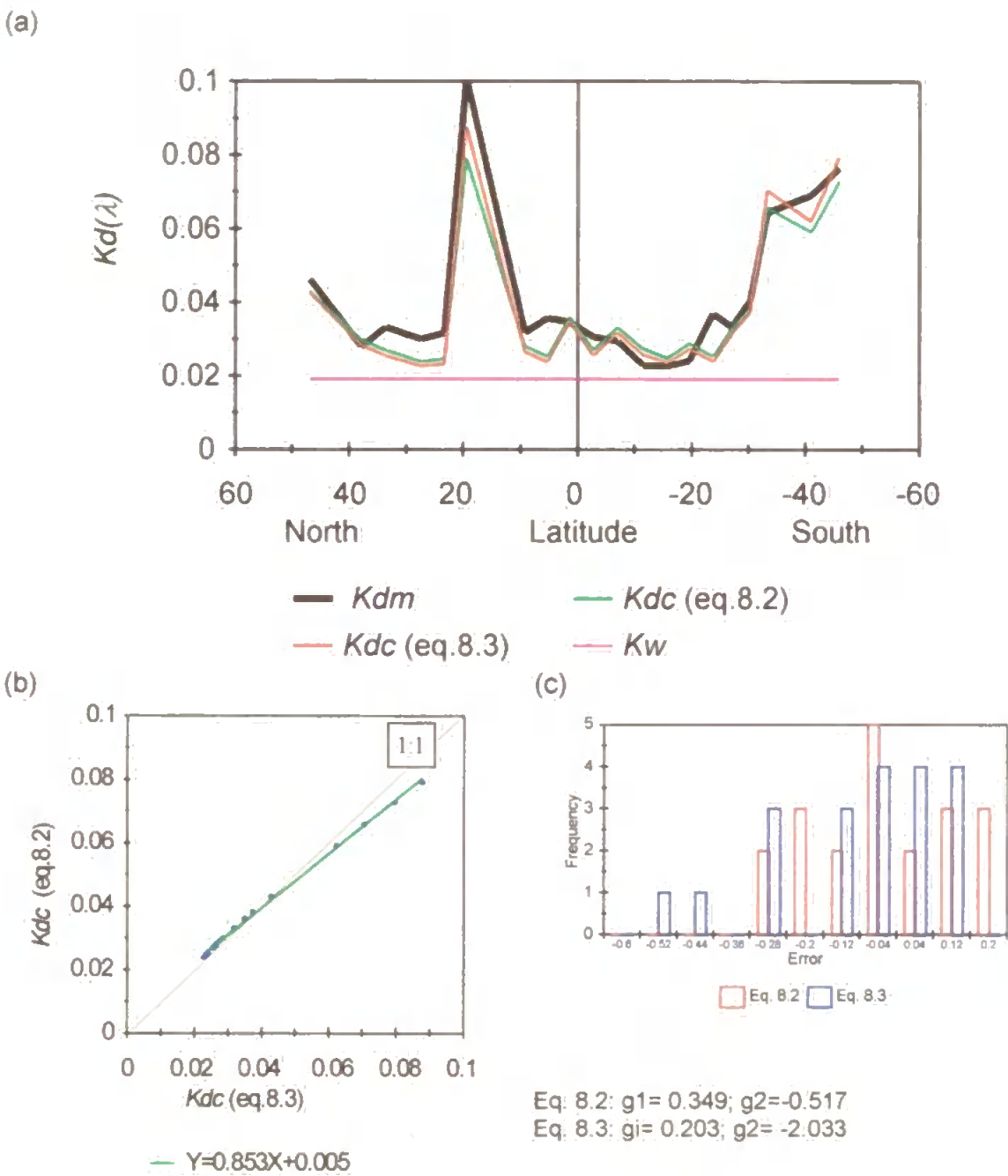
Figure 8.7 (a) Comparison and (b) regression analysis of the retrieved values of K_d(490\text{nm}) from equations 8.2 ( K_{dc}(490\text{nm}) this work) and 8.3 ( K_{dc}(490\text{nm}) Moore et al. , (1997)) for the AMT-1 data set. The units for K_d(\lambda) are \text{m}^{-1} . (c) shows a histogram of the frequency distribution of the errors.
