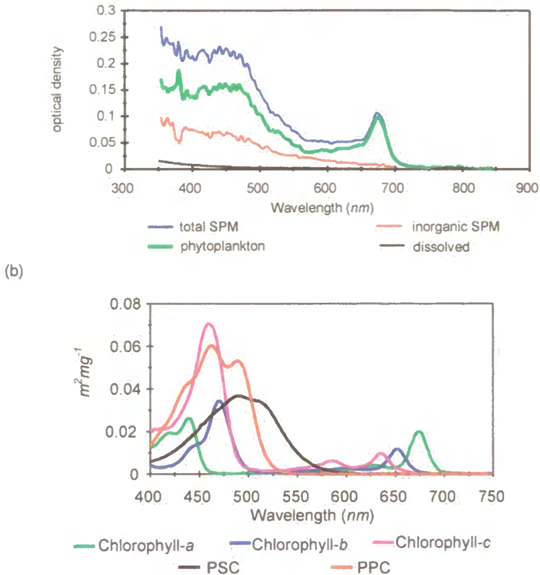
Figure 2.7. (a) An example of the absorption spectra of some constituents of a water sample collected at station L4 from a depth of 10m (1995, SDY 167). Data were determined from spectrophotometric analysis of a water sample concentrated on a Whatman GF/F filter pad (Mueller and Austin, 1995). DOM data were obtained from a sample filtered to 0.2\mu m (Kirk, 1980; Mueller and Austin, 1995). The biological fraction was removed using a hot methanol bath. Data were corrected to zero absorption at 750nm , but the path length amplification factor, \beta_L , had not been applied (Cleaveland and Weideman, 1993). (b) 'Unpackaged' specific absorption coefficient spectra of some pigments identified in this study: chlorophylls -a, -b and -c, and the carotenoids grouped as photosynthetic (PSC) and photoprotective (PPC) types according to Bidigare et al. , (1990).
