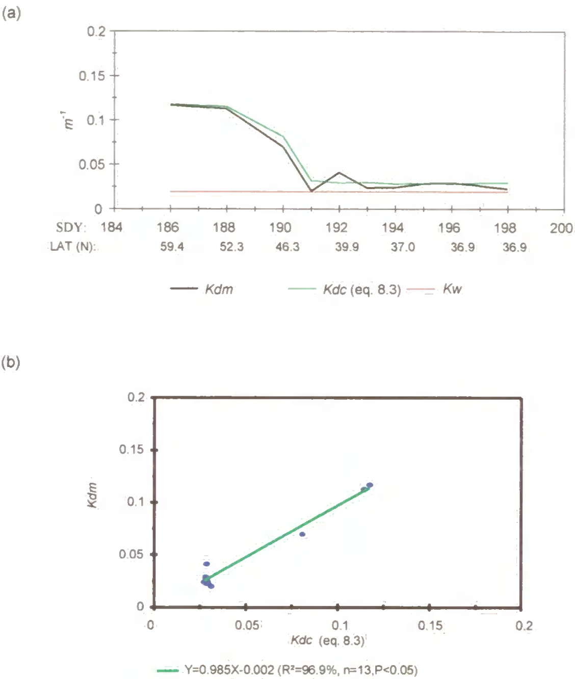
Figure 8.4 Comparison of the measured PRIME K_d(490nm) data against the calculated K_d(490nm) using equation 8.3 to test the K_d(490nm) derived from the Ed(490, z) profile values measured during the fieldwork sessions, denoted here by K_{dm} . The units of K_d(\lambda) are m^{-1} .
