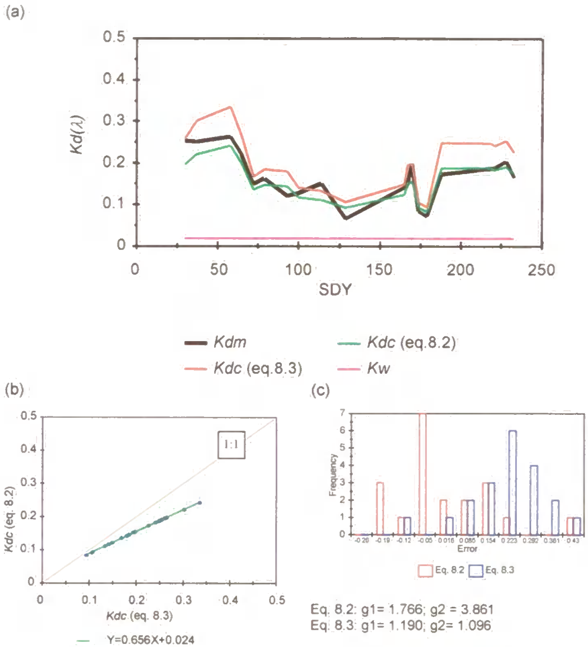
Figure 8.6 (a) Comparison and (b) regression analysis of the retrieved values of K_d(490nm) from equations 8.2 ( K_{dc}(490nm) this work) and 8.3 ( K_{dc}(490nm) Moore et al., (1997)) for the L4 data set. The units for K_d(\lambda) are m^{-1} . (c) shows a histogram of the frequency distribution of the errors.
