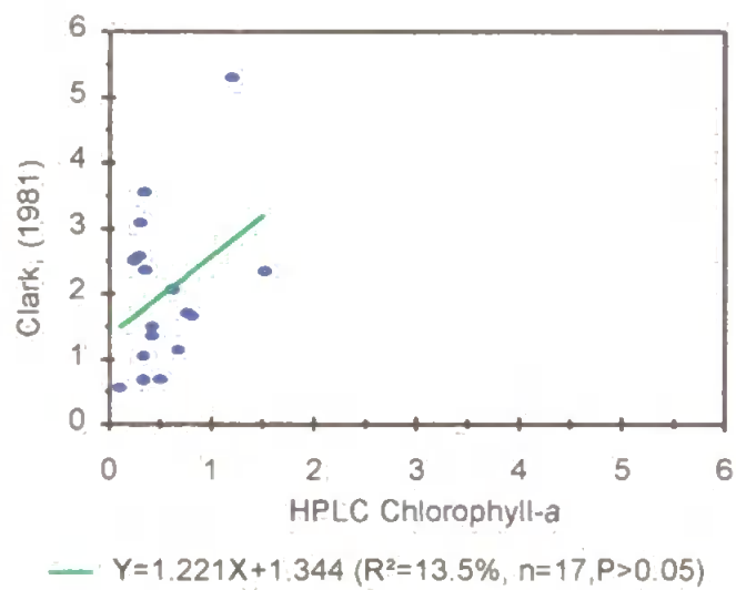
Figure 8.12 The CZCS pigment algorithm (equation 3.6) applied to the L4 data, showing both the phase similarity of the data and regression analyses between the measured and retrieved concentrations. The CHL-a concentration is in units of mg\ m^{-3} .
