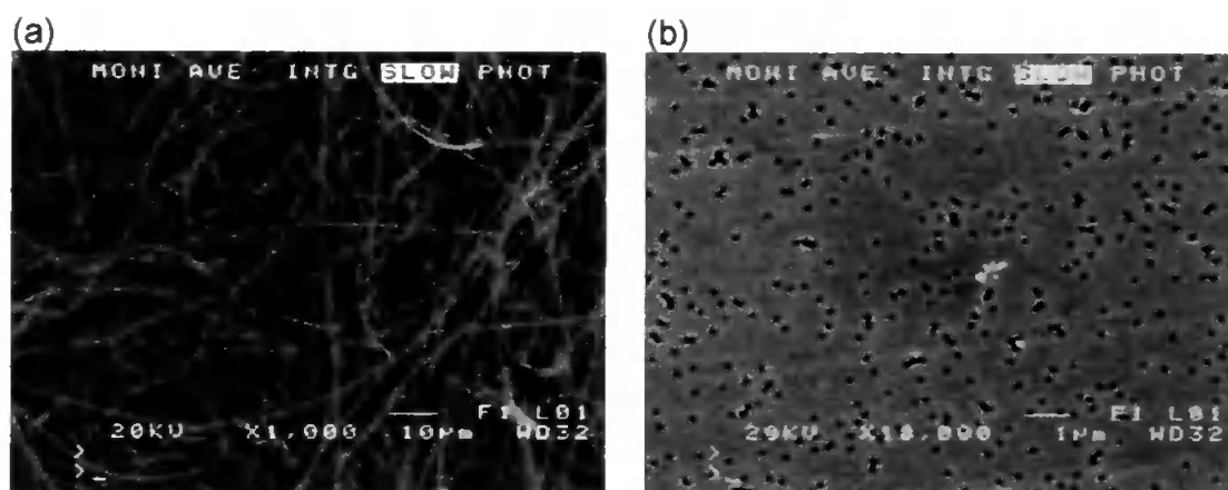
Figure 6.4. Scanning electron micrograph of (a) a Whatman GF/F ( 0.7\mu\text{m} ) glass fibre filter pad and (b) a 0.2\mu\text{m} Nulceopore membrane filter. Images generated courtesy of the University of Plymouth Electron Microscopy Unit.
