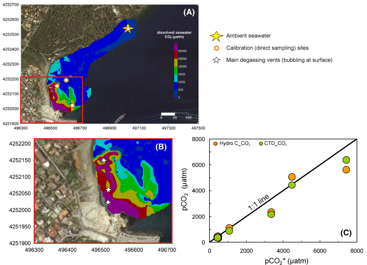
Fig. 9 a A map of seawater \text{pCO}_2 distribution in the Baia di Levante bay. The map was generated from in-situ real-time measurements of dissolved \text{CO}_2 , obtained using a HydroC TM sensor (for \text{CO}_2 < 6000 \mu\text{atm} ) and an Ocean Seven 303 IDRONAUT CTD (for \text{CO}_2 > 6000 \mu\text{atm} ). Measurements were obtained using a small boat and profiling along the track shown in Fig. 4 (bottom, right). The use of the HydroC TM and IDRONAUT CTD sensors to measurement of dissolved \text{CO}_2 in seawater was initially validated against results from conventional direct sampling, as shown in (c). Water samples for sensor comparison were collected in sites indicated by white circles; b a detail of (a). Stars identify the position of the main degassing vents (where gas bubbling at the free seawater surface was also concentrated); c comparison between \text{pCO}_2 values measured by
