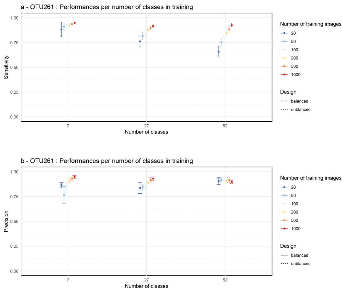
Figure 5-5: a) Differences in sensitivity for OTU261 in classifier trained with different number of classes and images (7 for group A, 27 for group B and 52 for group C). Error bars are standard deviation calculated from the 10 random splits. b) Differences in precision for OTU261 in classifier trained with different number of classes and images. Error bars are standard deviation of the 10 random splits
