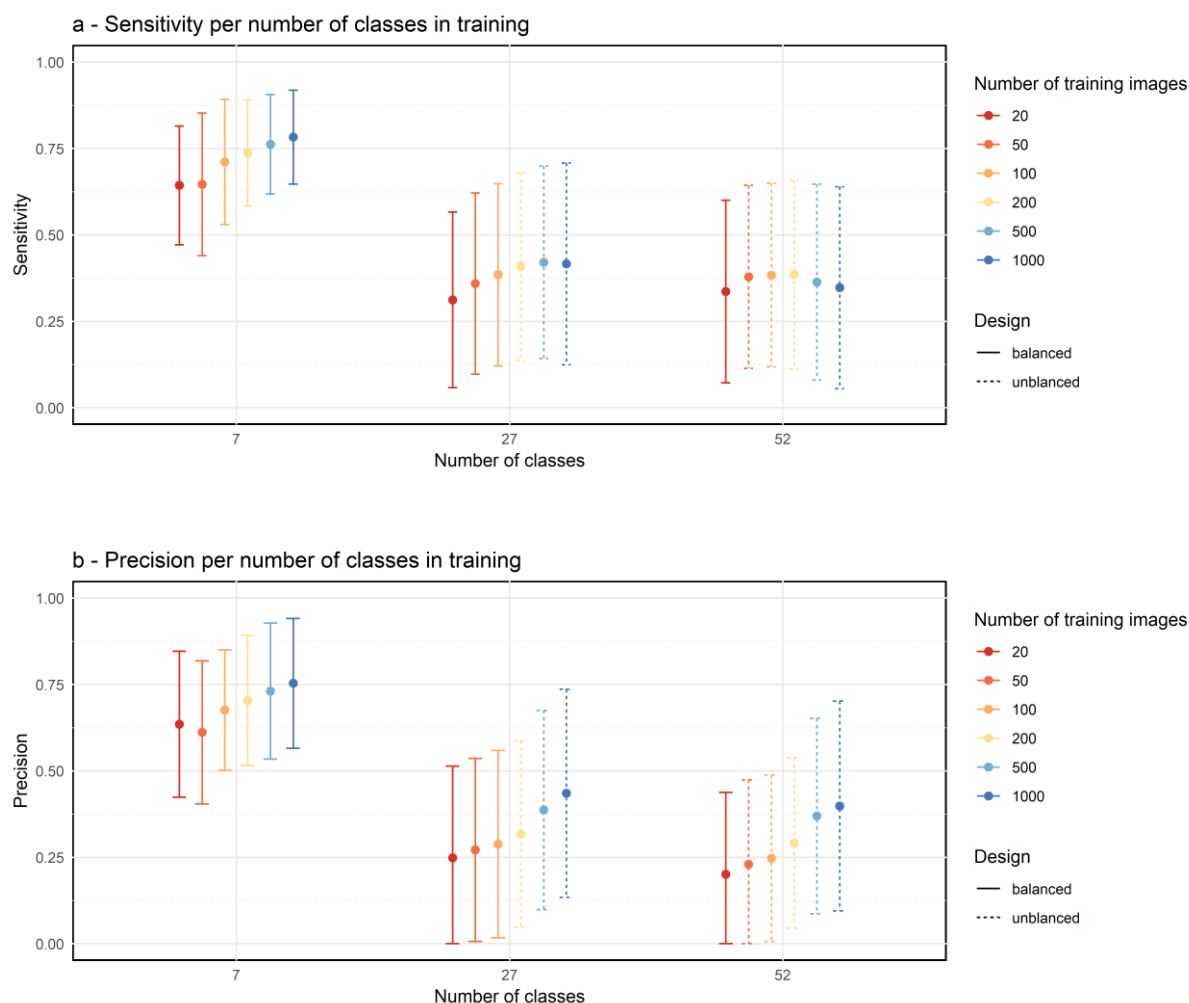
Figure 5-4: a) Differences in sensitivity in classifiers trained with different number of classes and images (7 for group A, 27 for group B and 52 for group C). b) Differences in precision in classifier trained with different number of classes and images. Error bars are standard deviation of the 10 random splits.
