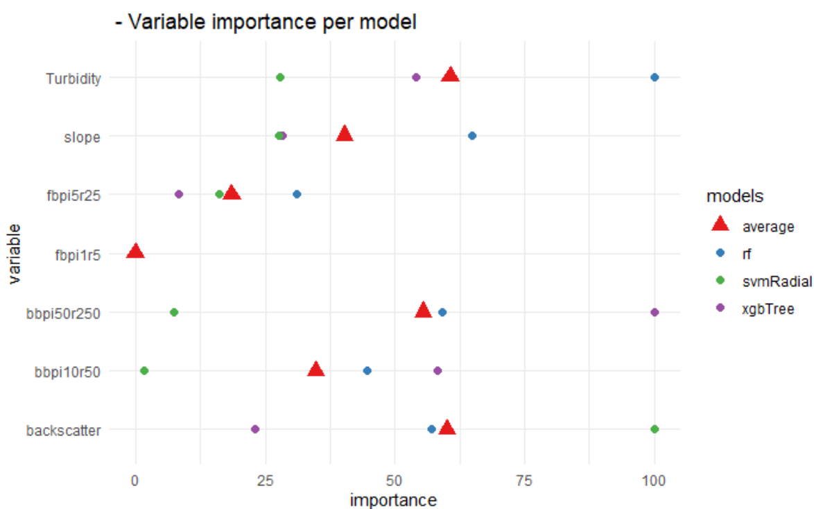
Figure 4-6: Relative variable importance plots of the ensemble model trained on all the data. Points are coloured by algorithms (rf: Random forest, svmRadial: Support Vector Machine, xgbTree: Extreme Gradient Boosting) and their average importance is displayed as red triangles. The higher the score the more important the variable is.
