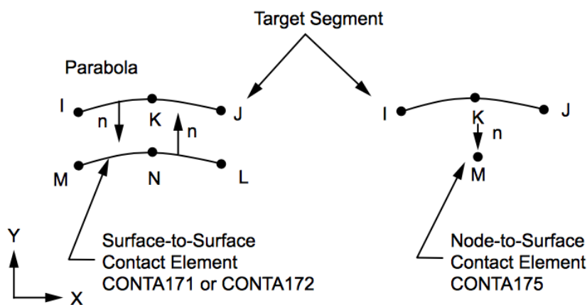
Figure 8: TARGE169 Geometry
