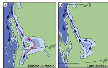
Fig. 7. Reconstruction of marine water circulation in the Sundance Seaway. A) Middle Jurassic, characterised by an arid climate system, with southward flow into the seaway (blue arrows) of isotopically light, surface marine waters from the Arctic region, and northward flow of more saline and denser (red arrows) Sundance Seaway waters. B) Late Jurassic, characterised by a semi-arid and winter-ice conditions, with a northward flow of less dense Sundance Seaway waters (blue arrows) that would inhibit the southward surface flow of ocean waters into the seaway.
