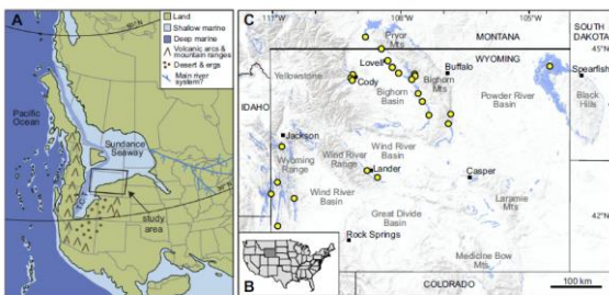
Fig. 1. Palaeogeographic reconstruction of western North America in the Middle Jurassic showing the Sundance Seaway and study area (A) and location map of the study area (B, C). A, modified from Blakey, 2014. Localization of desert, ergs and mountain ranges from Kocircak and Dott Jr. (1983); presence of a hypothetical transcontinental river from Dickinson and Gebre (2009).
