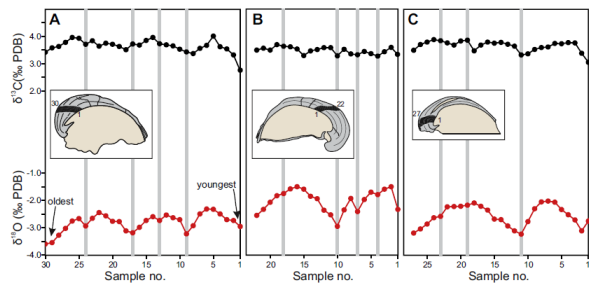
Fig. 5. High-resolution carbon and oxygen isotope record across three specimens of Gryphaea nebrascensis . Grey lines indicate dark bands on the shells which identify breaks in shell accretion (see Supplementary Fig. S3).
