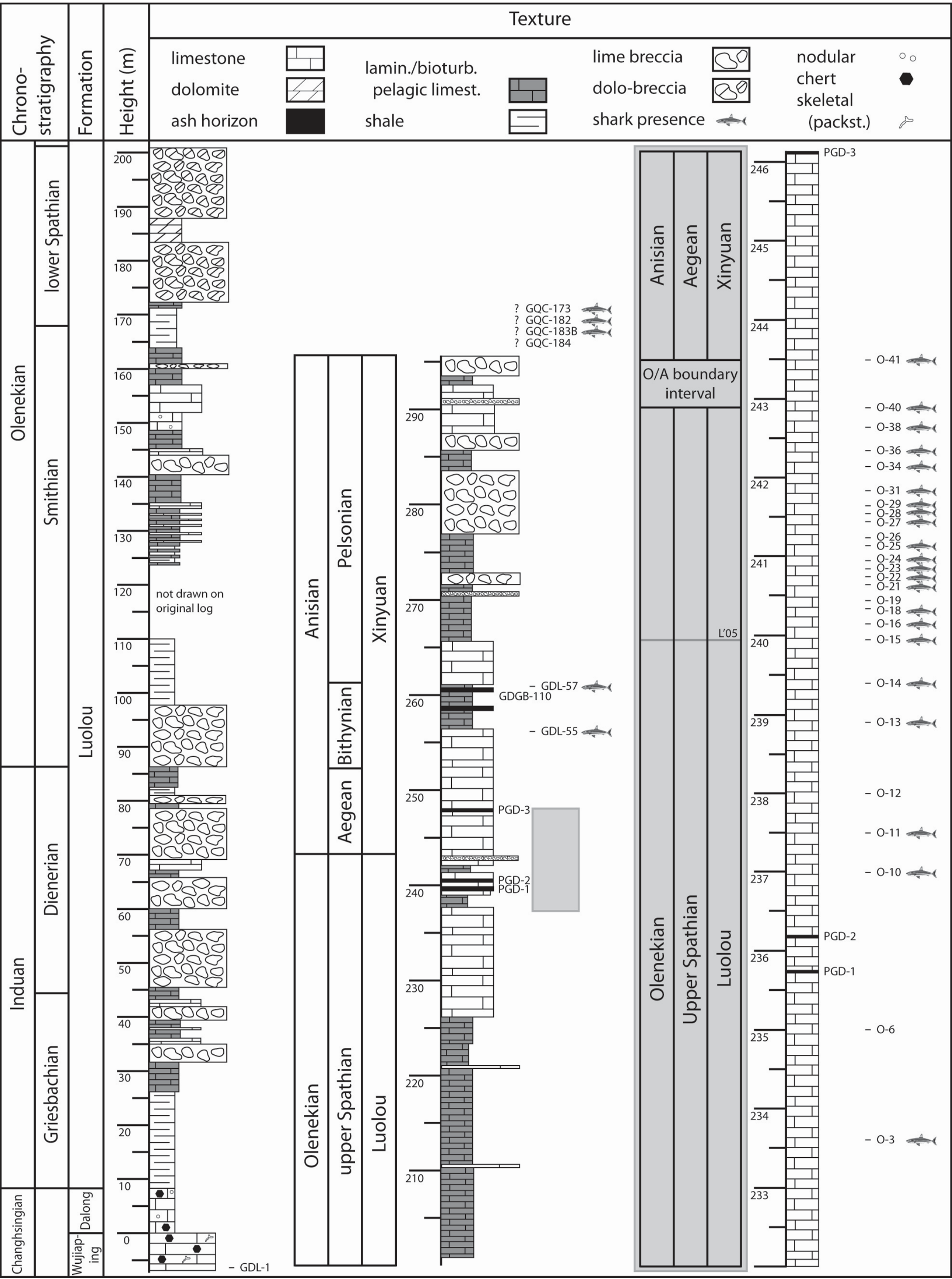
Figure 4.7, p.171 in KOOT, M. B. 2013. Effects of the Late Permian mass extinction on chondrichthyan palaeobiodiversity and distribution patterns. unpublished PhD thesis, 853 pp., Plymouth University.
