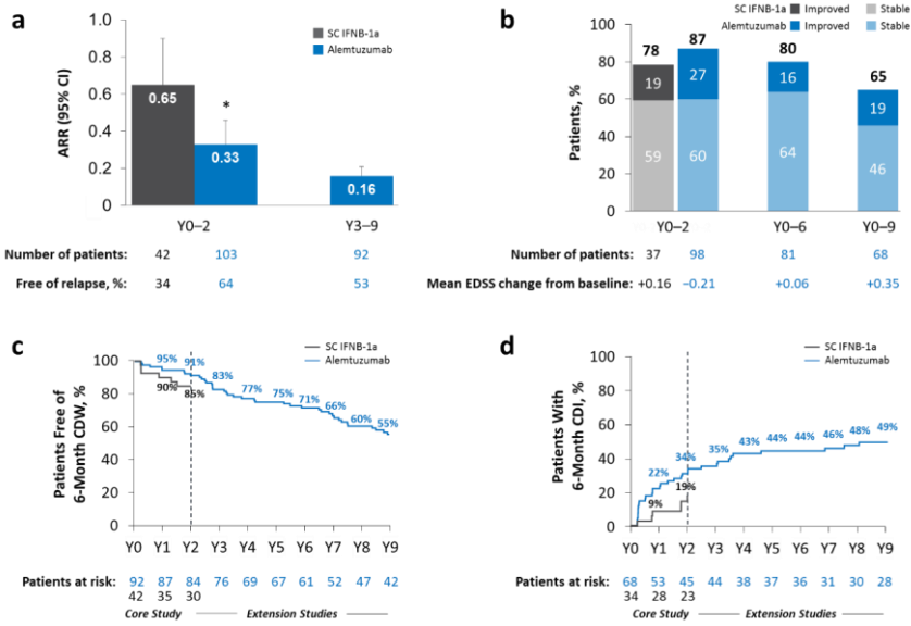
Fig. 3 Clinical efficacy in CARE-MS II alemtuzumab-treated HAD patients through Year 9: (a) ARR; (b) percentage of patients with improved or stable EDSS scores over time; (c) percentage of patients free of 6-month CDW; (d) percentage of patients achieving 6-month CDI
