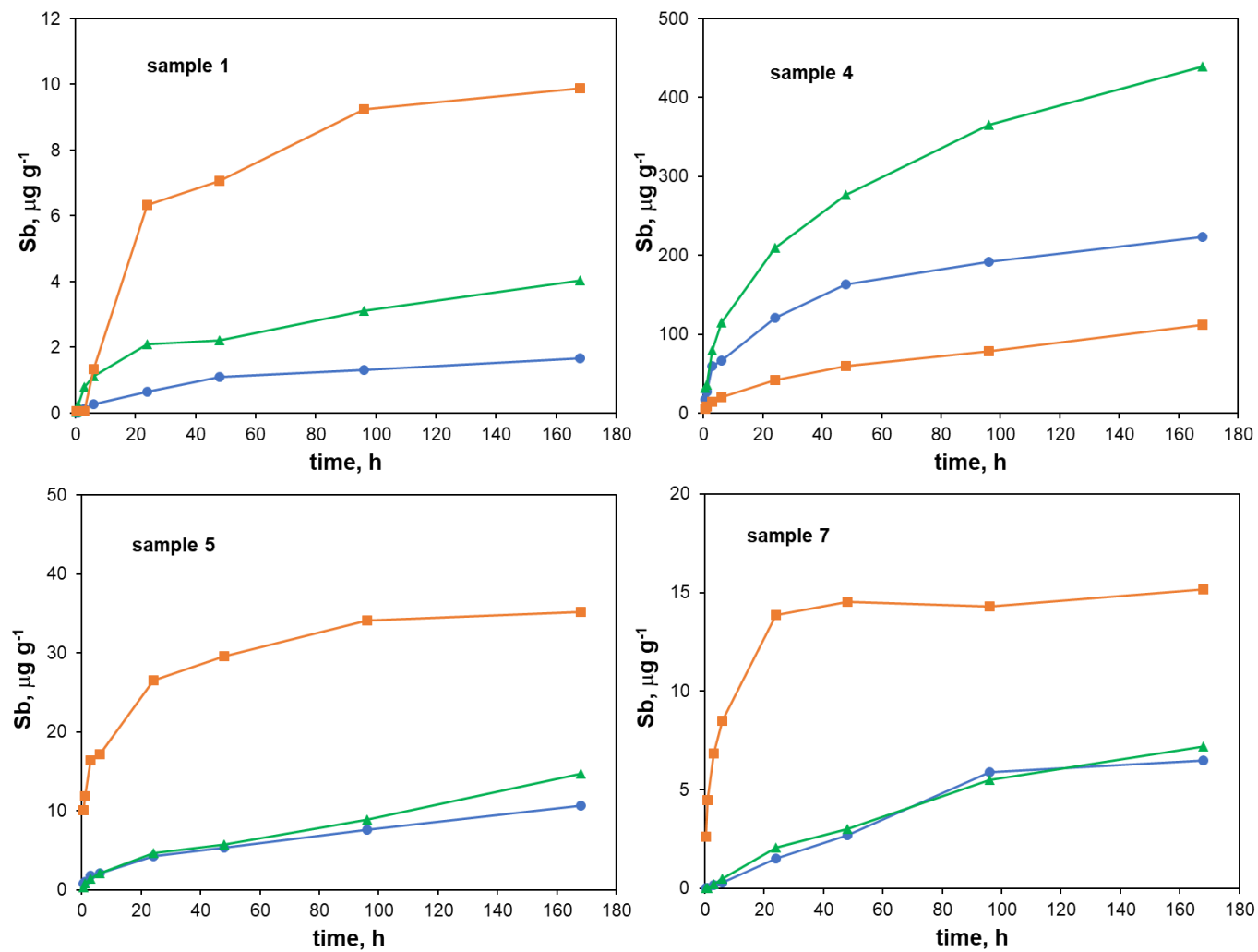
631 Figure 6: Mobilisation of Sb from micronised plastic samples as a function of time in NaCl solution (blue circles), the PBET (green triangles) 632 and DA-PBET (orange squares). 633 634 635
