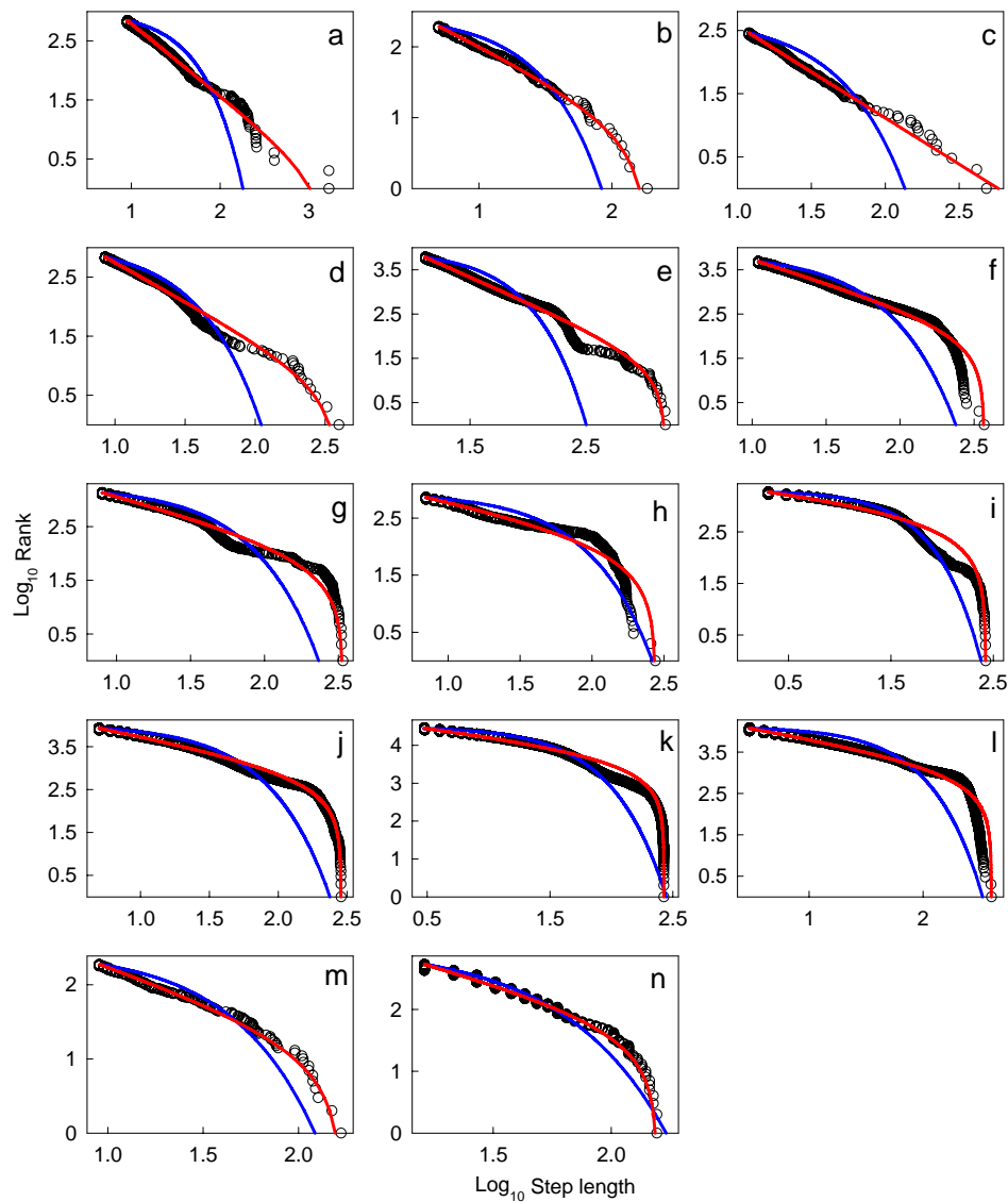
Figure S3. Ranked step-length plots for sections well fitted by a truncated Pareto-Lévy distribution.
