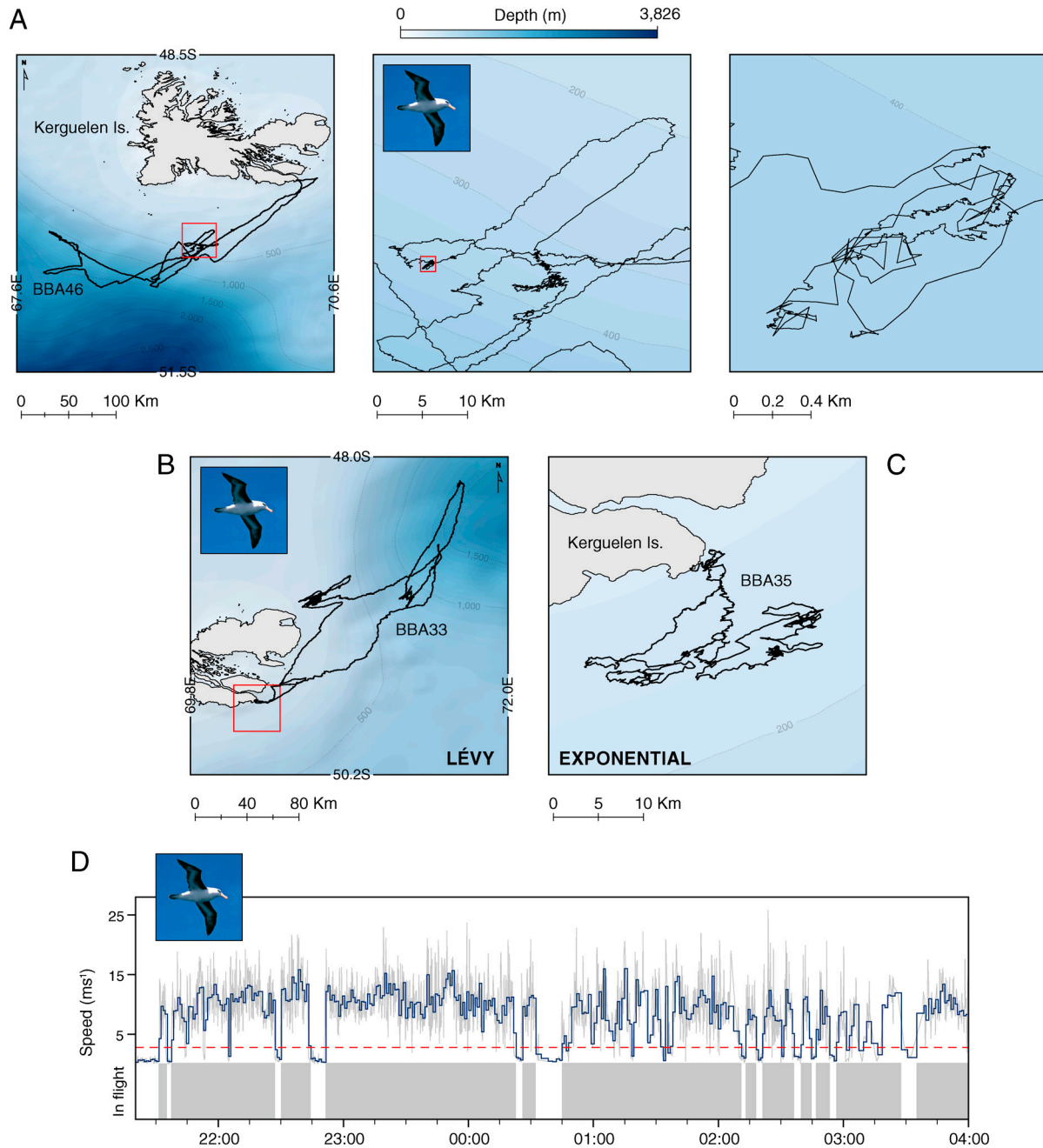
Fig. 1. GPS trackings of albatross foraging indicate scale-invariant patterns. (A) GPS foraging track of a black-browed albatross (BBA46) off the Kerguelen Islands, Southern Indian Ocean, viewed across large (100 s km; Left) to small (10 s m; Right) scales showing similar patterns of trajectory complexity at all scales. Background color denotes bathymetry in m. Each red square denotes area covered by panel adjacent right. (B) Foraging track of a black-browed albatross (BBA33) with flight steps between landings best approximated by a truncated Lévy distribution ( \mu = 1.28 ), with movements principally in deep shelf and oceanic habitats. Red square denotes area shown in (C). (C) Foraging track of BBA35, best approximated by an exponential distribution, was more spatially intensive in shelf and shelf edge habitats. Color denotes water depth, with bathymetric contours identifying neritic shelf waters <2,000 m and oceanic waters >2,000 m. (D) Time series profile of flight speeds of a GPS tracked black-browed albatross showing how landing locations and surface resting times were identified.
