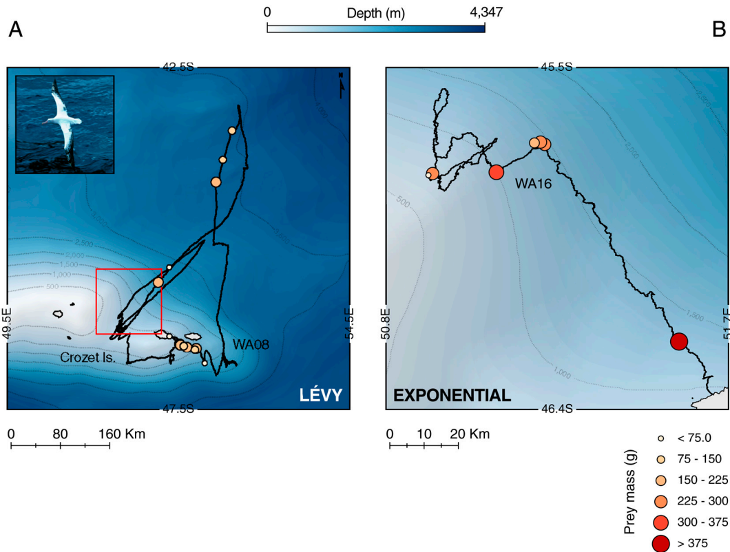
Fig. 2. Different types of wandering albatross GPS tracks and prey capture contrasts between Lévy and exponential patterns. (A) Foraging track, prey capture locations, and prey masses of wandering albatross WA08 during an 89 h foraging trip approximated by a Lévy pattern ( \mu = 1.25 ) occurring principally over deep shelf edge (1,000–2,000 m) and oceanic waters (>2,000 m). Captures totalled 3.5 kg, but prey were generally solitary and taken further apart, indicating prey sparse habitats. Red square denotes area shown in (B). (B) Foraging movements by wandering albatross WA16 during which it captured 1.8 kg of prey in 21.5 h when over shallow shelf (500–1,000 m) and shelf edge habitats during landings best described by an exponential distribution (Brownian pattern). Numerous prey items were often taken in a single landing, indicating a greater abundance of prey.
