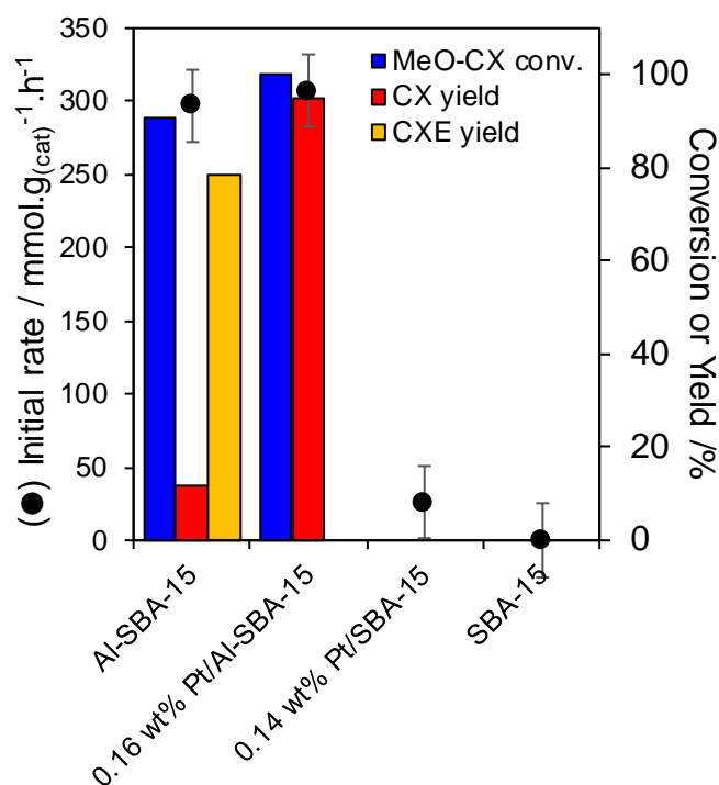
Figure 7. Comparison of activity, and 6 h conversion and product yields for methoxycyclohexane hydrodeoxygenation over SBA-15, Al-SBA-15 and Pt analogues. Reaction conditions: 200 °C; 20 bar \text{H}_2 ; 25 mg 0.14 wt% Pt/SBA-15 or 0.16 wt% Pt/Al-SBA-15; 10 mmol methoxycyclohexane; 50 mL n-dodecane solvent; and 800 rpm.
