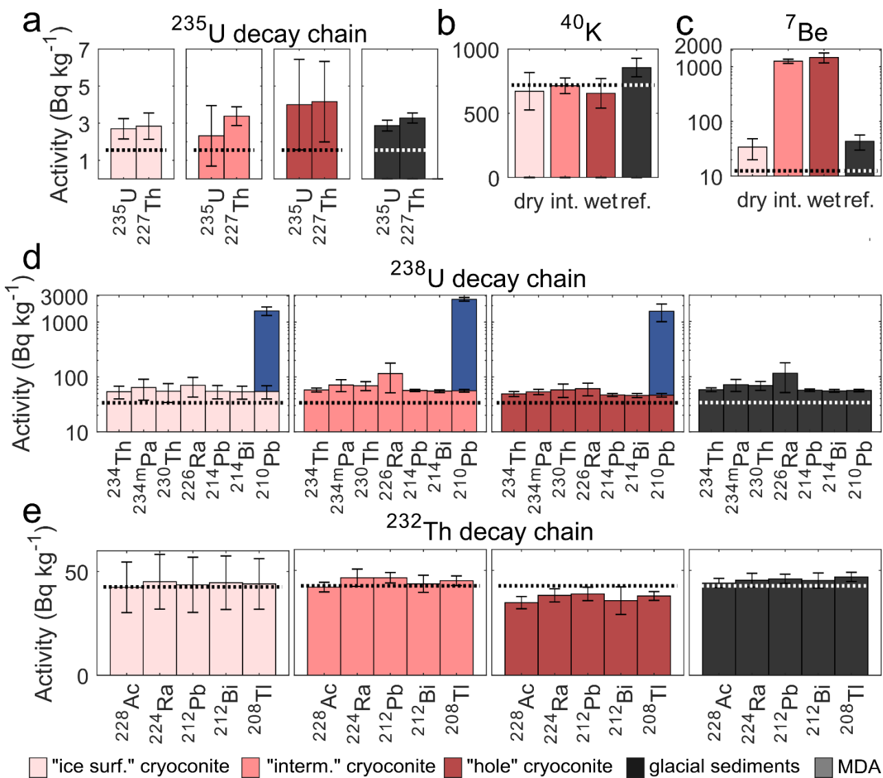
Fig. 2 Natural radionuclides in cryoconite samples from the Morteratsch glacier. Data refer to "ice surface", "intermediate" and "hole" cryoconite types, and to proglacial sediments (sed.) collected near the glacier terminus. The dashed line corresponds to average UCC activities, calculated from the reference by Rudnick & Gao (2003). The reference for ^7\text{Be} is taken from Mabit et al. (2008). ^{210}\text{Pb} activity is represented for both 255 supported (red shades) and excess fractions (blue).
