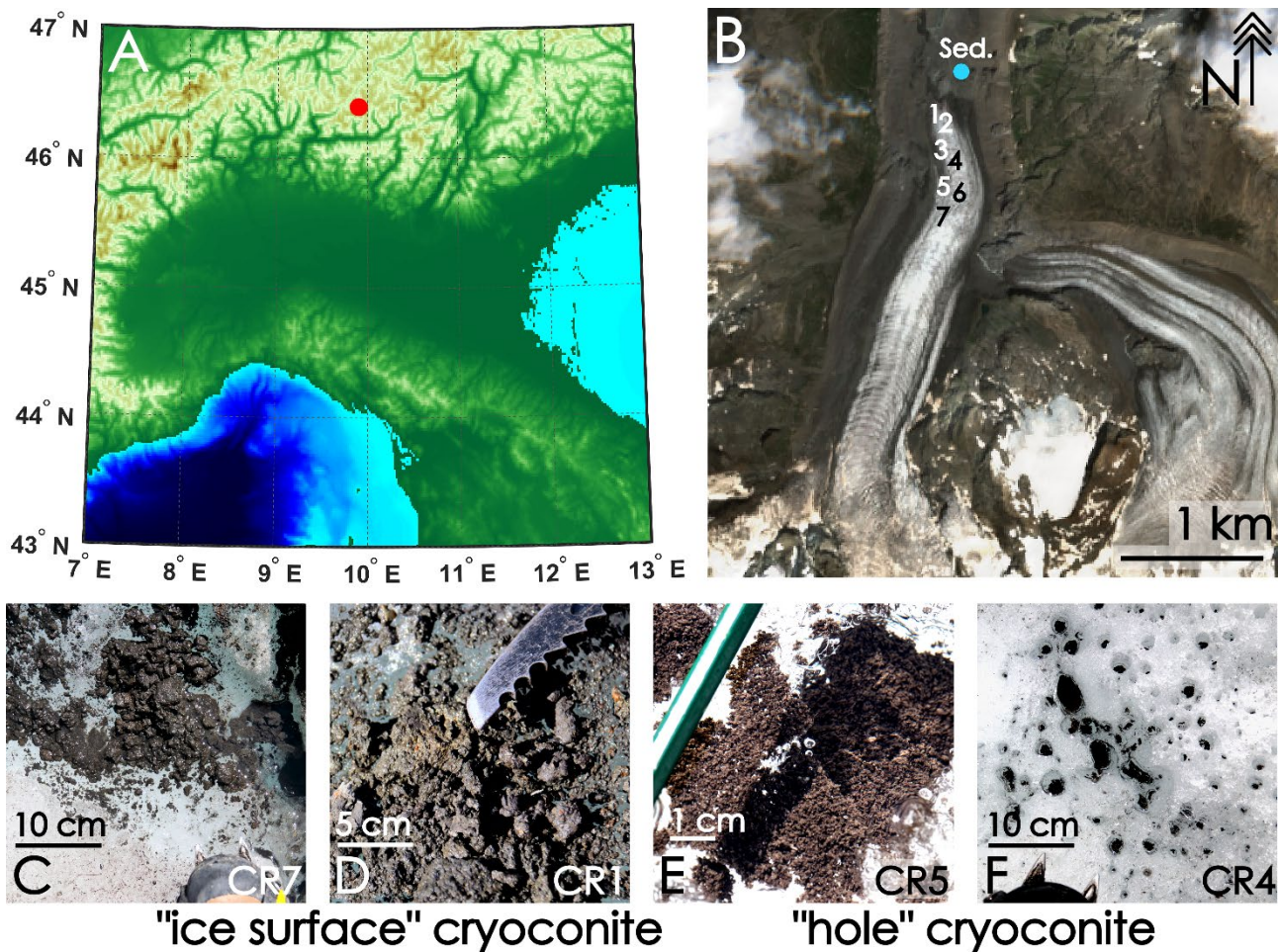
135 Fig. 1 The geographic setting of the present study. The relief map (panel A) shows the position of Vadret da Morteratsch within the Alps (red dot). In panel B a satellite picture of the glacier is presented (Sentinel 2, ESA), retrieved on July 16 th , 2018. Sampling sites are highlighted by numbers corresponding to cryoconite sample codes, and by a blue dot (riverine proglacial sediments). In the lower row, examples of cryoconite samples belonging to the “ice surface” (C,D) and “hole” (E,F) types are shown.
