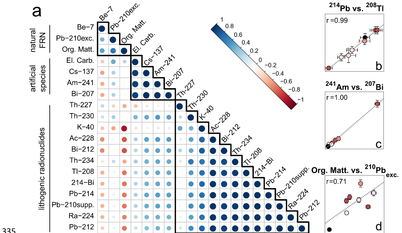
335 Fig. 4 Correlation among the variables considered in this study. In panel a the correlation is illustrated using a Pearson's correlation matrix where correlation coefficients are represented by circles whose color and size depend on their value. Variables have been ordered and clustered into three groups, following a hierarchical clustering approach. Clusters are defined by black solid lines. Panel b-d: linear correlation between selected variables belonging to the three clusters; the same color palette of Fig. 2 has been used. 340
