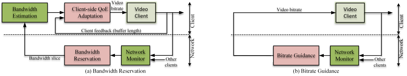
Fig. 13: QoE-based network-assisted approaches for adaptive video streaming. (a) A specific bandwidth for each client is enforced by the network when bandwidth reservation is used, and (b) the network provides an explicit bitrate to the clients using bitrate guidance [107].
