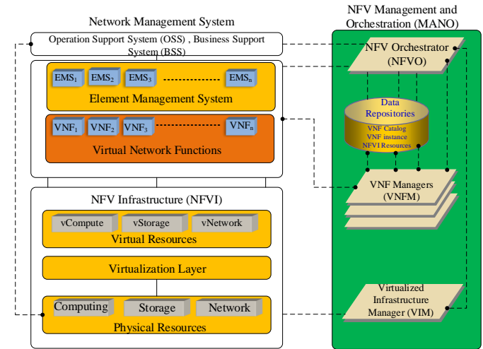
Fig. 12: The ETSI NFV MANO framework.
