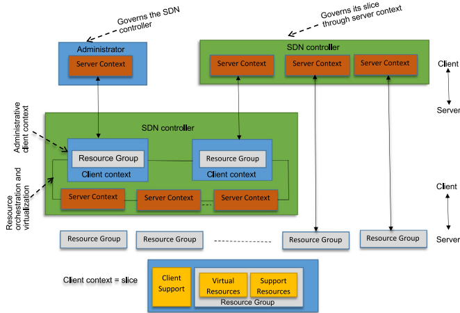
Fig. 9. ONF SDN network slicing architecture [86].
