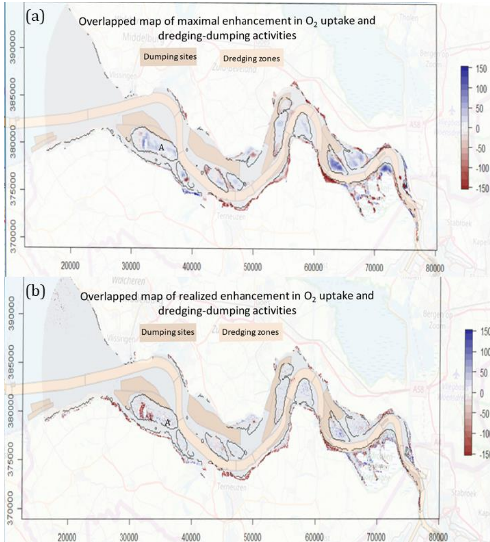
Figure 5.6: Overlapped maps of temporal variation (2010-1955) in (a) maximal and (b) realized faunal-mediated O 2 uptake (in mmol m -2 d -1 ) of tidal submersion and dredging-dumping activities summarized until 2010 ( http://www.scheldemonitor.be ). Symbol A is the tidal flat Hooe Platen, where the adverse effects were predicted by upper quantile and full quantile scenarios.
