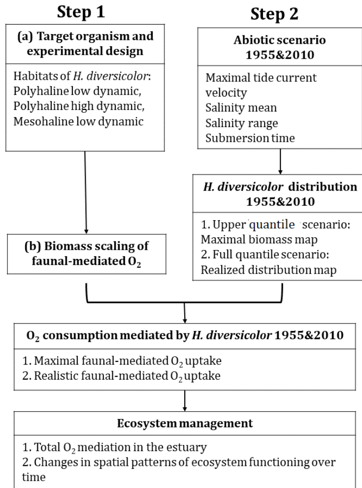
Figure 6.4: Schematic of the 2-step model integration (Chapter 5). Experimental measurements and biomass-scaling of faunal-mediated O 2 uptake (Step 1) is composed of (a) Target organism and experimental design and (b) biomass-dependent faunal-mediated O 2 uptake; Step 2 is to extrapolate ecosystem functioning over quantile regression model by adopting a mixed modelling approach with two temporal scenarios 1955/2010.
