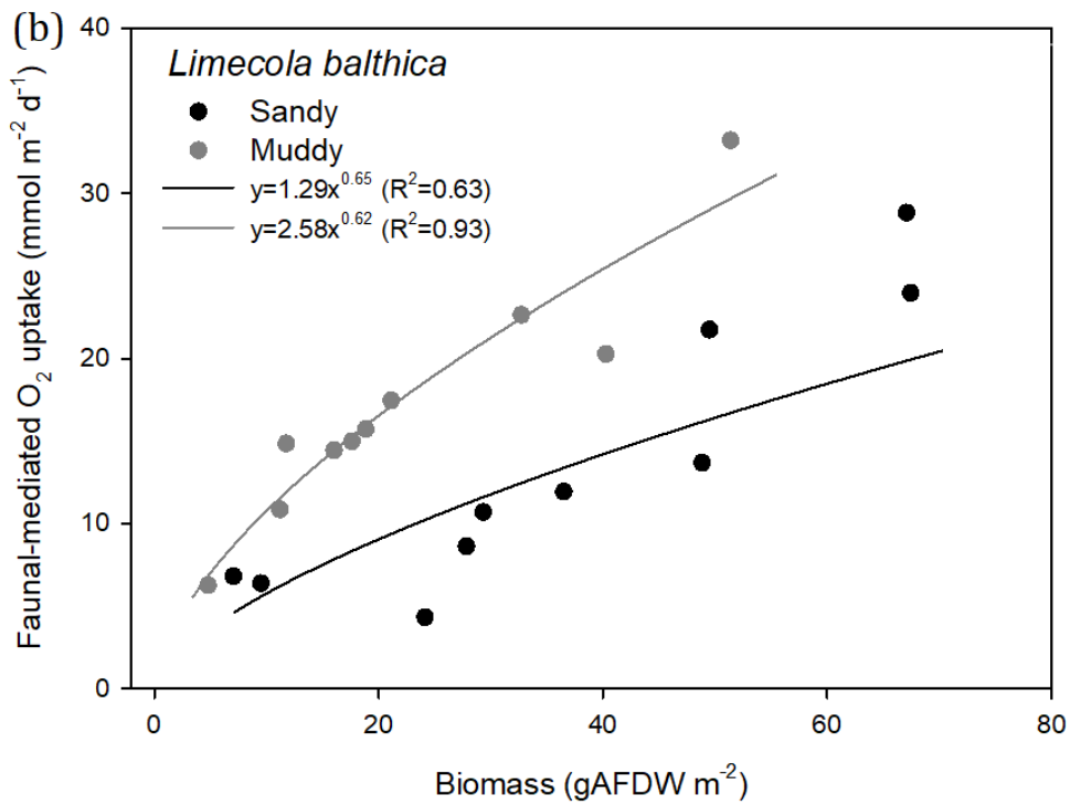
Figure 4.3 Faunal-mediated O 2 uptake (mmol m -2 d -1 ) measured in each microcosm as a function of animal biomass (AFDW), and the best-fit power functions ( p < 0.05 ) for (a) H. diversicolor and (b) L. balthica .
