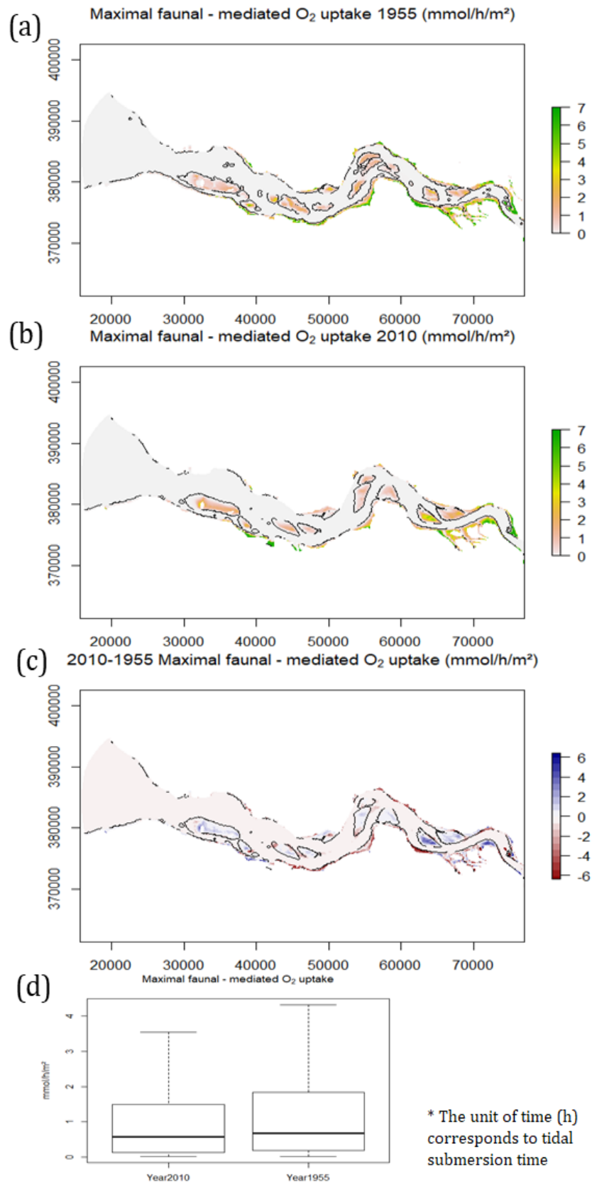
Figure 5.4: Maximal faunal-mediated O 2 uptake (mmol m -2 h -1 ) during tidal submersion in the Western Scheldt in (a) 1955, (b) 2010, (c) Difference over the time span \Delta_{2010-1955} , and (d) Temporal comparison (1955 vs 2010) of the faunal-mediated O 2 uptake estimated from the upper quantile distribution (potential niche) of H. diversicolor (Quantile regression, tau=0.95). Symbol (C) showed the location of the drastic spatial variation in O 2 uptake.
