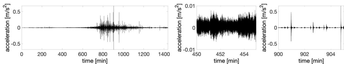
Figure 13: Wolf Rock acceleration response during ex-Hurricane Ophelia, 16 th October 2017. Left, for the whole day, middle for 7.30AM (low tide), right for 3PM.
