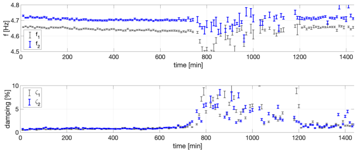
Figure 16: Wolf Rock monitoring. Frequency estimation (upper) and damping estimation (lower) from application of BAYOMA to data of Figure 16.
