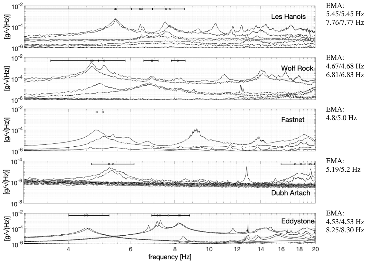
Figure 6: Singular value decomposition of averaged ambient response data spectra, with corresponding mode frequencies identified by experimental modal analysis (EMA) of shaker test data with arbitrary orthogonal axes. Error bars indicate frequency bands manually chosen for BAYOMA identification and circles indicate BAYOMA-identified mode frequency (most probable values).
