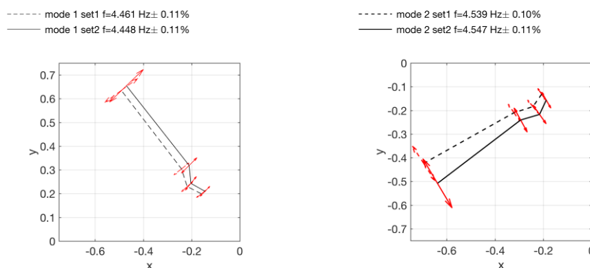
Figure 12: Eddystone first pair of modes for upper level ordinates.
