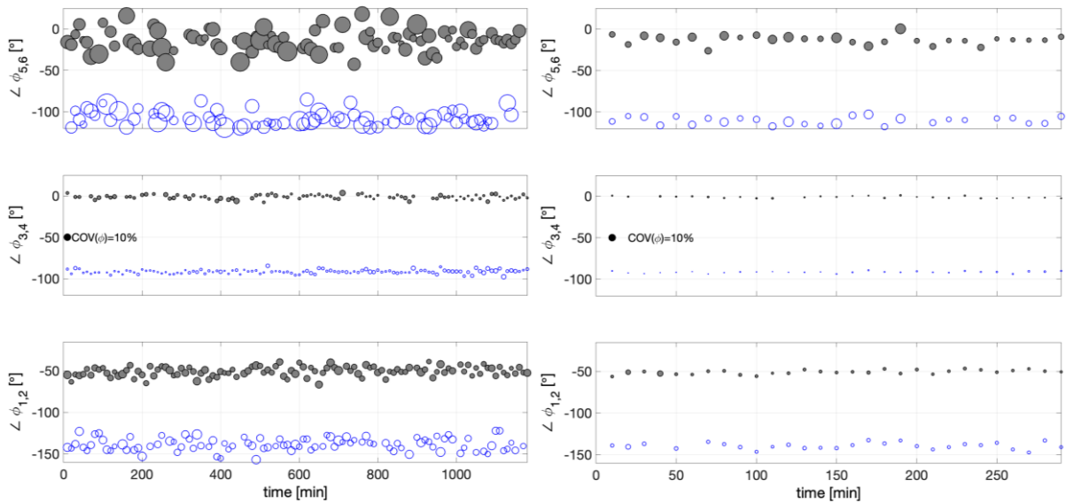
Figure 15: Mode shape variation for (bottom to top) first, second and third mode shape pairs corresponding to Figure 14. Size of circles reflects 1\sigma identification uncertainty on individual estimate.
