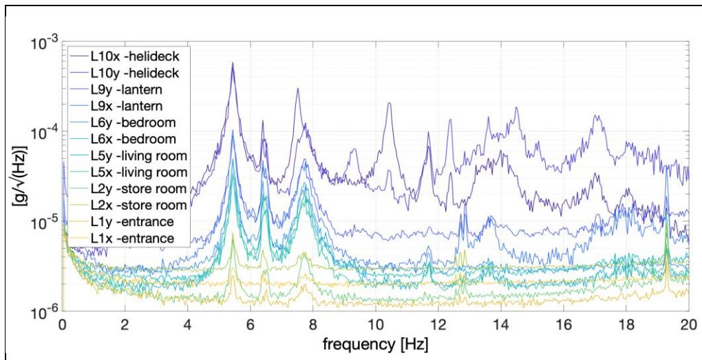
Figure 5: Les Hanois Lighthouse ambient response power spectral density
