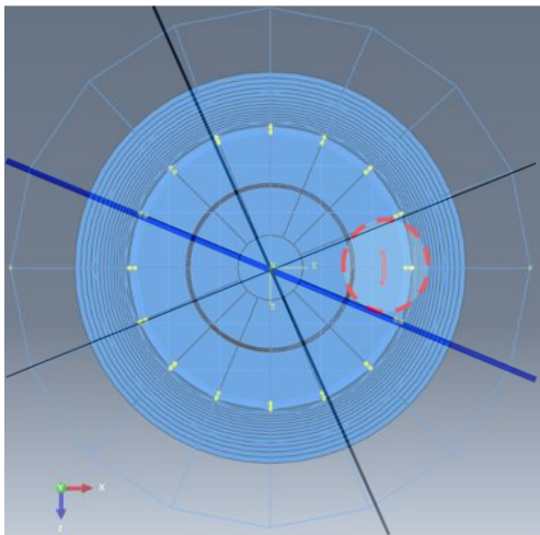
Figure 10: Wolf Rock first (left columns) and second (right columns) mode pairs. Level 9 (upper) and 8 (middle). FEM modes (lower), red curve locates upper door. (Thick) blue lines are in direction of landing platform (also the entrance).
