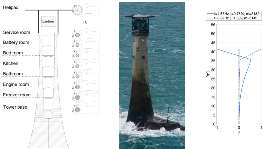
Figure 2: Wolf Rock Lighthouse. Vertical section through tower, accelerometer angles; aerial view of lighthouse and landing area; EMA modes. Photo: James Bassitt
