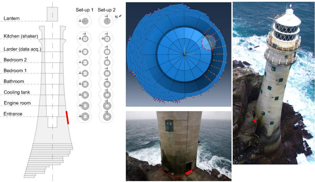
Figure 3: Fastnet Lighthouse: (left) vertical section through structure and accelerometer arrangements in two sets, (mid upper) FEM showing door, (mid lower) view of rock restraint from stump of old tower, (right) drone view showing extended courses. Measurement x axis is through door, FEM x axis is rotated 22.5° clockwise from door. Photos: James Bassitt and Athanasios Pappas.
