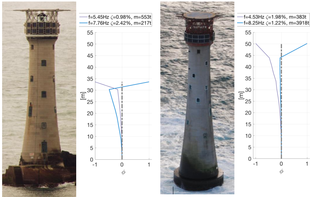
Figure 1: Les Hanois (left) and Eddystone (right) Lighthouses and first two modes identified from experimental modal analysis of forced vibration test data for nominal x direction. Photos: Emma Hudson (left), Trinity House (right).
