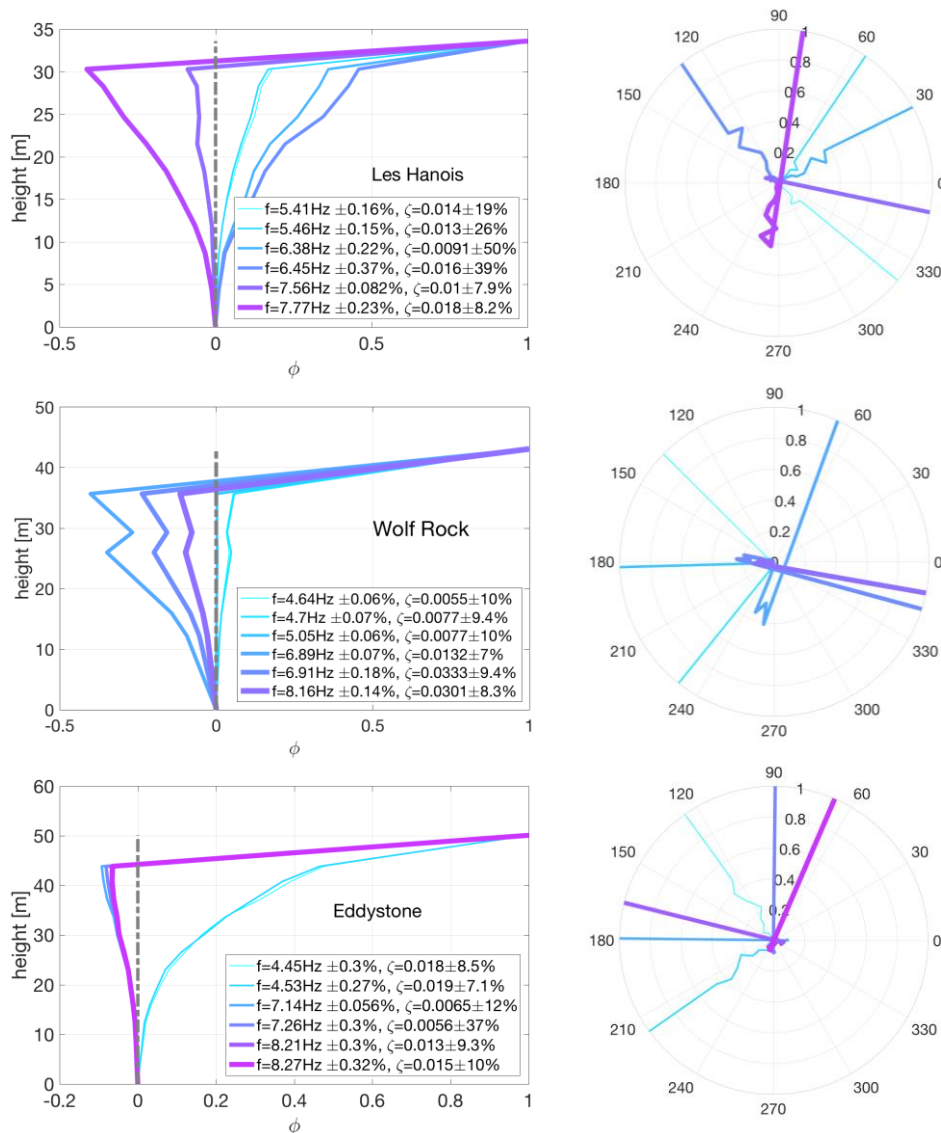
Figure 8: BAYOMA modes. Left elevation, rotated to same plane; right in plan.
