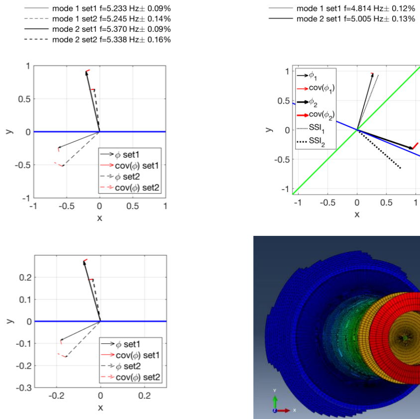
Figure 11: Left column Dubh Artach level 7 (upper) and level 3 (lower); x axis (blue line) is aligned with openings (windows, doors). Right column Fastnet; x axis aligns with entrance, green line is North-South axis, blue line is x axis of FEM. FEM second mode, along the model axes shown bottom right.
