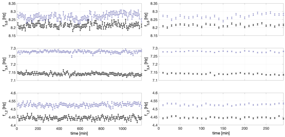
Figure 14: Mode pair frequency variation for overnight recording at Eddystone Lighthouse.
