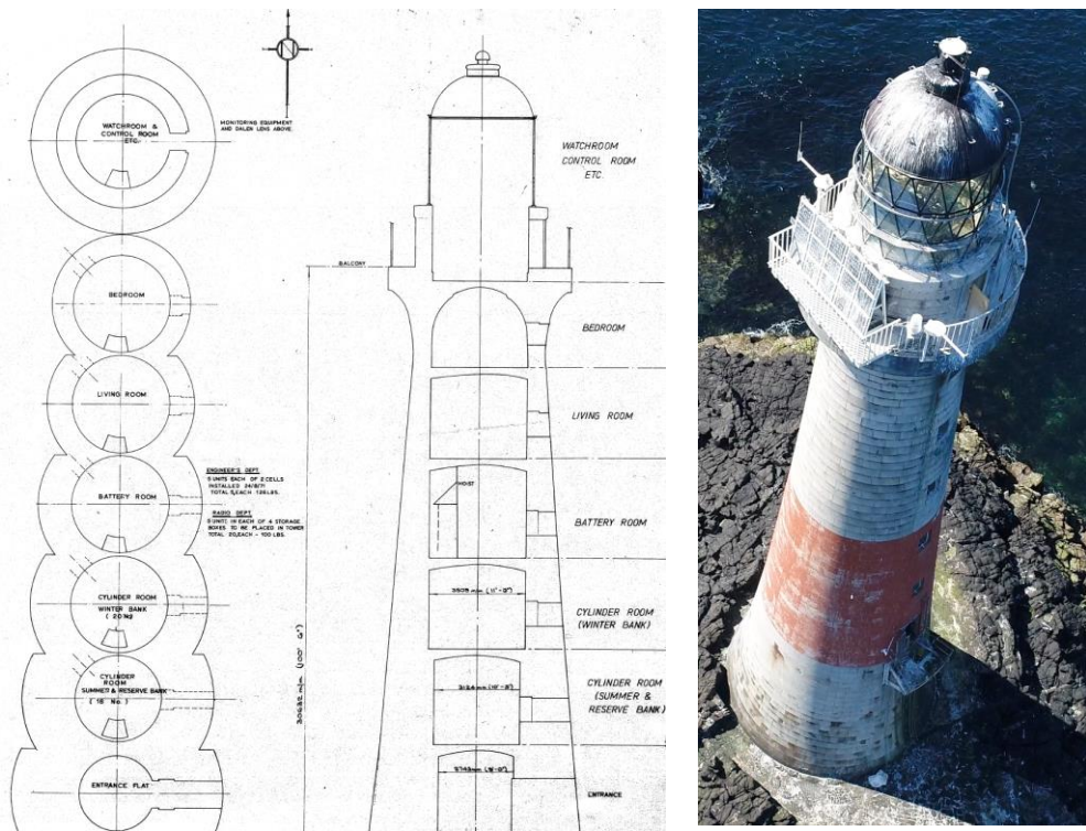
Figure 4: Dubh Artach Lighthouse horizontal and vertical sections and aerial view, showing alignment of openings. Photo: James Bassitt, drawings courtesy of Trinity House.
