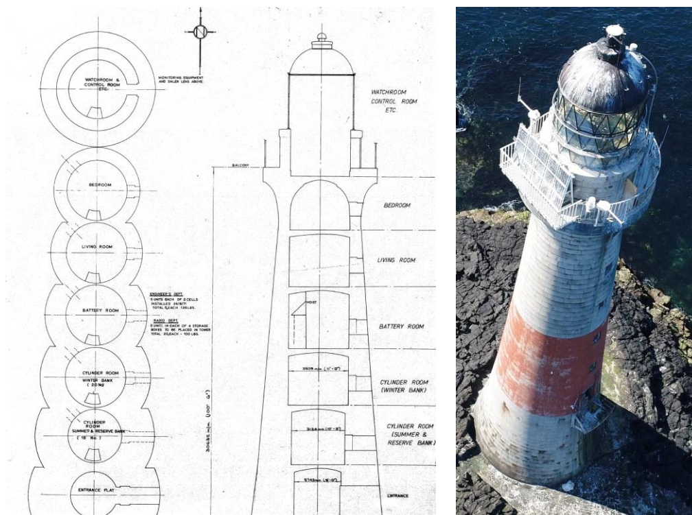
Figure 4: Dubh Artach Lighthouse horizontal and vertical sections and aerial view, showing alignment of openings. Photo: James Bassitt, drawings courtesy of Trinity House.
