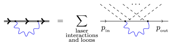
FIG. 2. One-loop correction to the double line representation.
