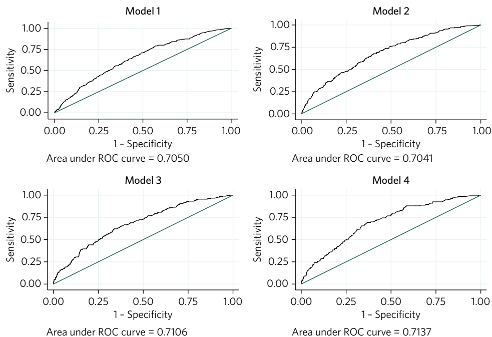
Fig. 1 Receiver operating characteristic (ROC) curves for logistic regression models 1-4.
