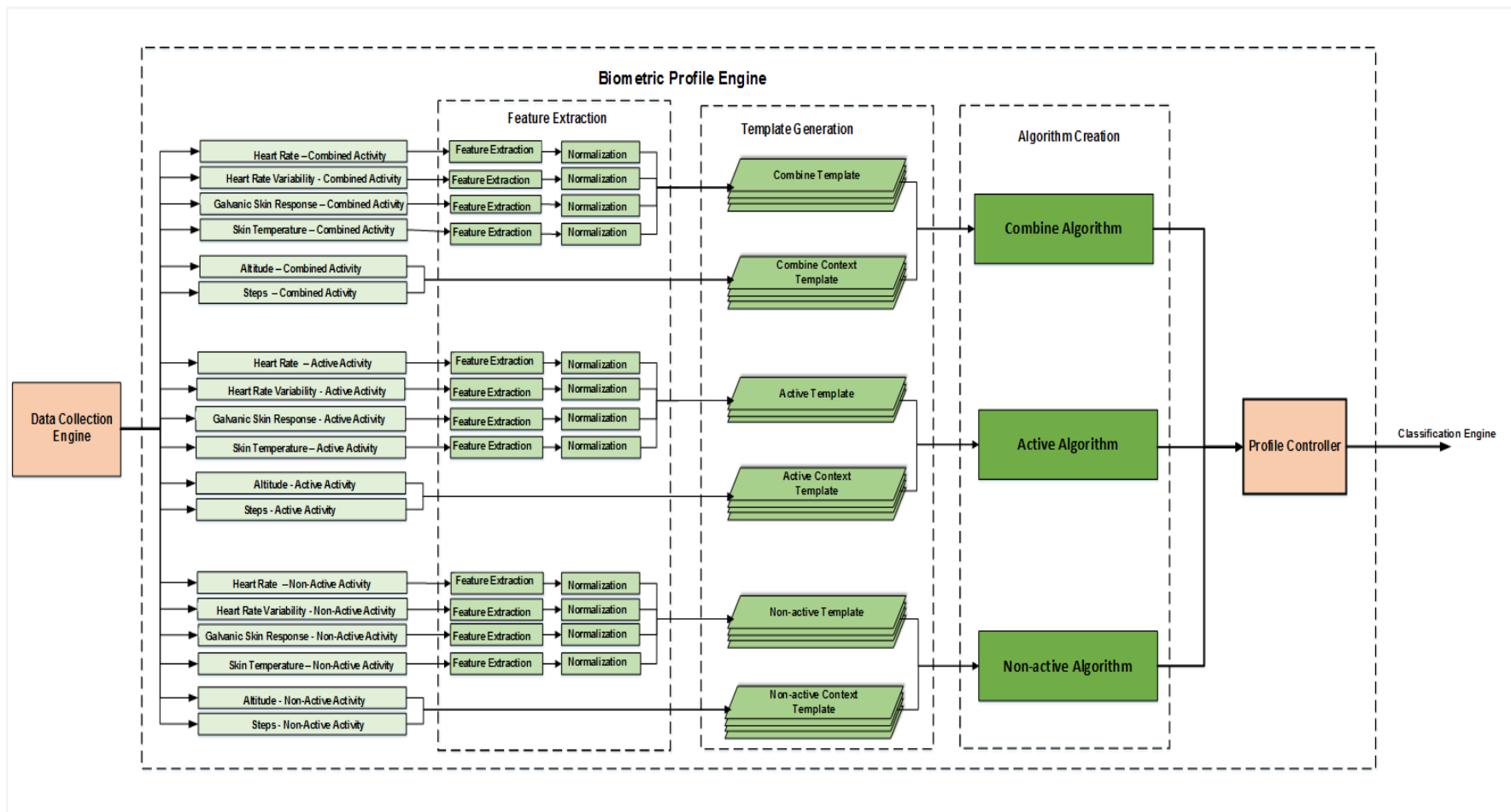
Figure 6. 4: Biometric Profile Engine
