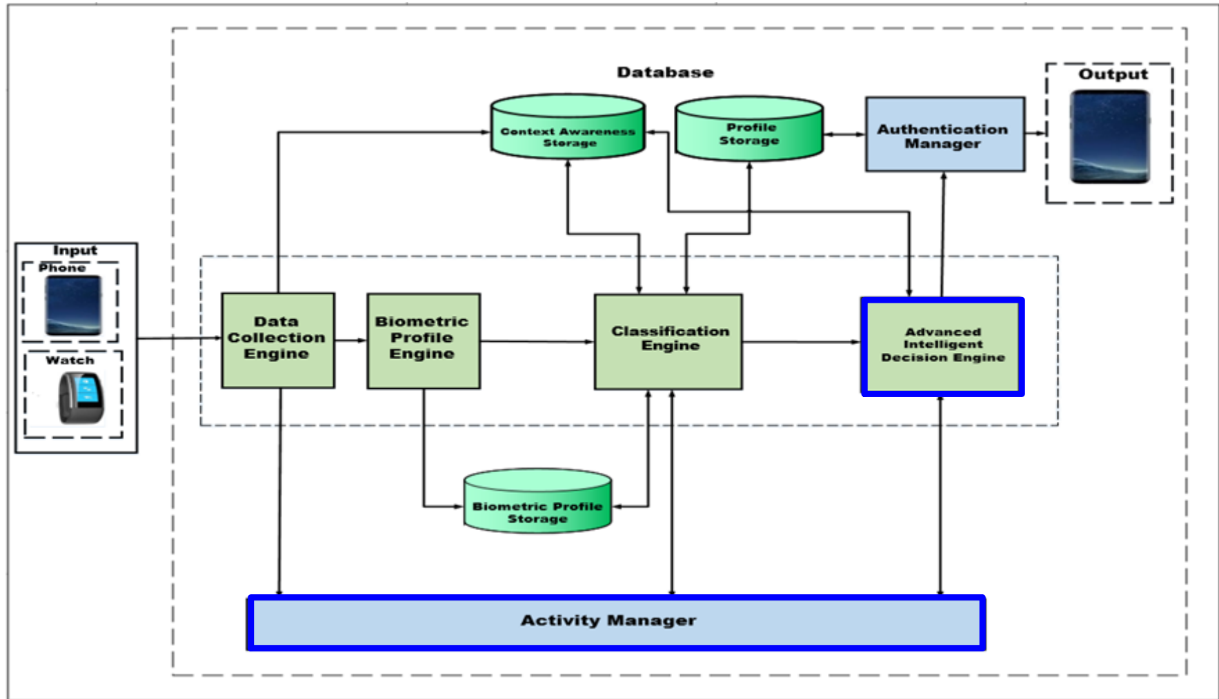
Figure 6. 1: A Novel Bioelectrical Body Recognition Framework showing the added layers with blue borders
