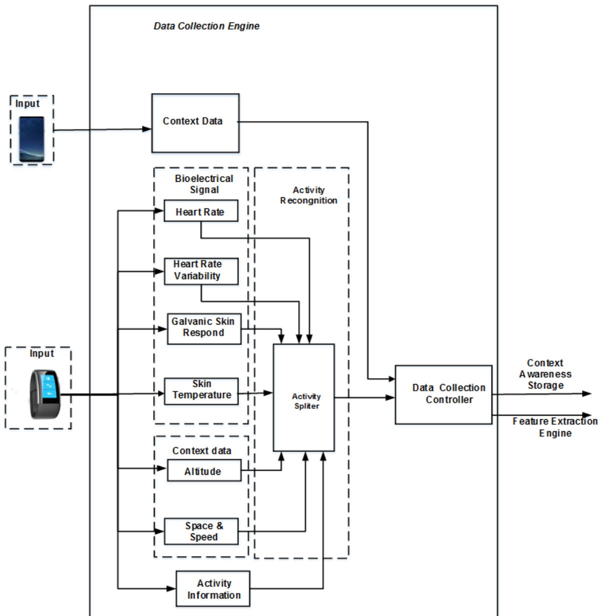
Figure 6. 2: Data Collection Engine
