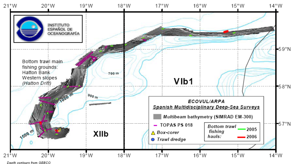
Figure 3.3.2 Preliminary map showing the sampling carried out during the ECOVUL/ARPA Spanish Multidisciplinary Deep-Sea Surveys (2005-06) on the Hatton Bank. The study area covers main trawl fishing grounds. These grounds are located on western slope of the Bank, between 1000-1500m depth, mostly over the soft sedimentary deposits called Hatton Drift.
