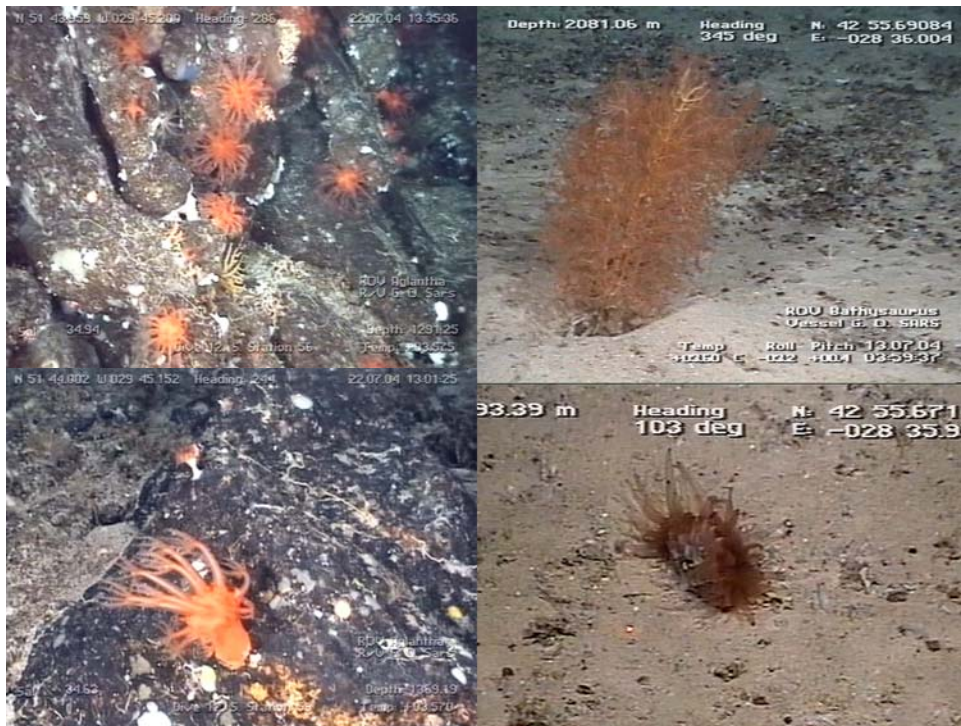
Fig 7.3.6.1 Examples of two common habitats along the MAR. Left) Exposed basaltic outcrop with a high abundance of the alcyonarian Anthomastus sp. Right) Soft, sandy sediments with scattered shells or pebbles, Acanella arbuscula (upper right), and Flabellum alabastrum (lower right) (figure from Mortensen et al. in press)
