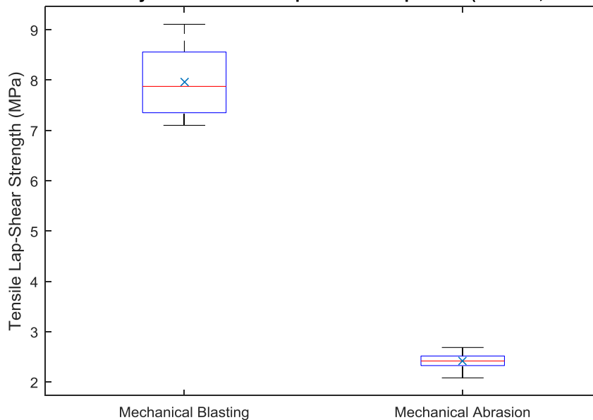
Figure 15: Statistical analysis 5 and 6, showing surface preparation comparisons for a composite adherend thickness of 10 plies. Statistical analysis 5 specimens were manufactured by adhesive bonding. Statistical analysis 6 specimens were manufactured by co-curing.
