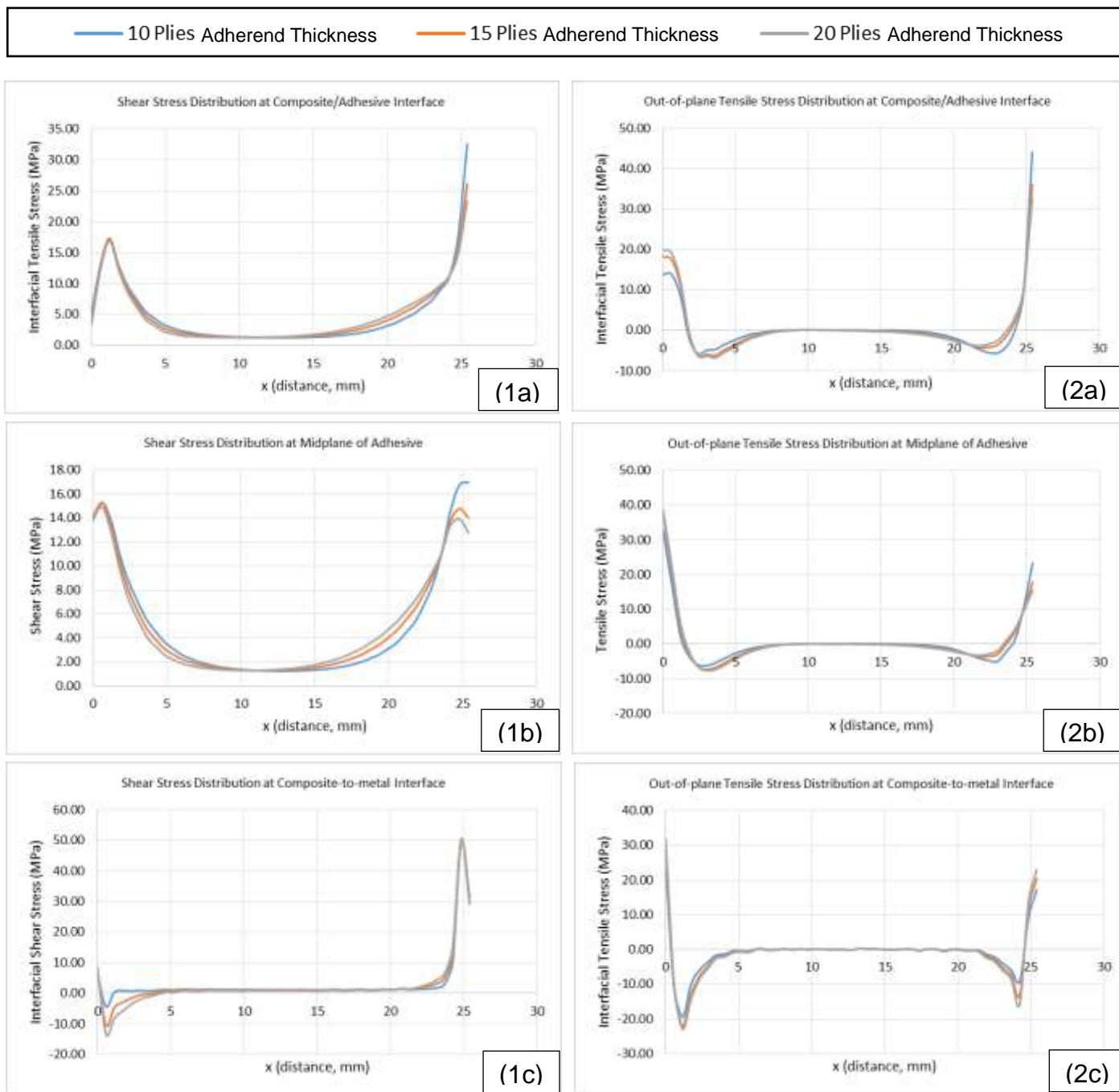
Figure 9: Numerical results for shear (1) and out-of-plane tensile (2) stress distributions. For adhesively bonded joints, stress distributions were obtained at (a) the composite-adhesive interface and (b) along the midplane of the adhesive layer. For co-cured joints (c), results were obtained at the composite-to-metal interface.
