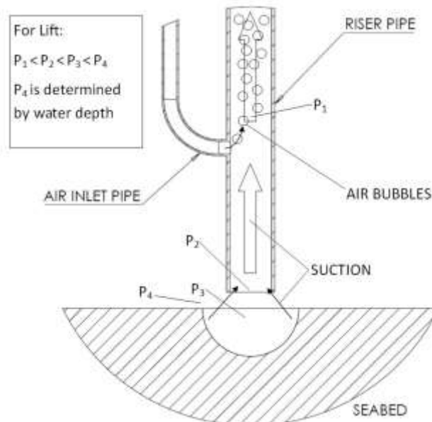
Figure 3; Basic Pressure Requirements for Airlift Pumping
