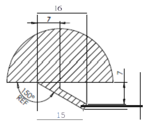
DETAIL C SCALE 2:1
