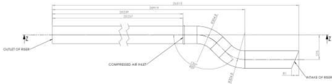
Figure 2 -The Riser Drawn With Dimensions from Figure XX (Hackwell, 2015)
