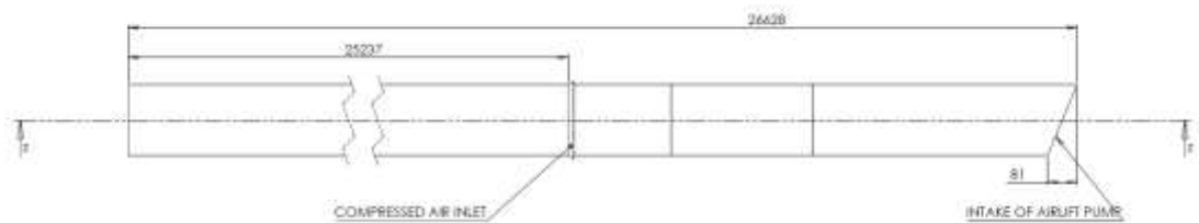
Figure 3 - The Riser Drawn With Dimensions from Figure XX (Hackwell, 2015) Simplified
