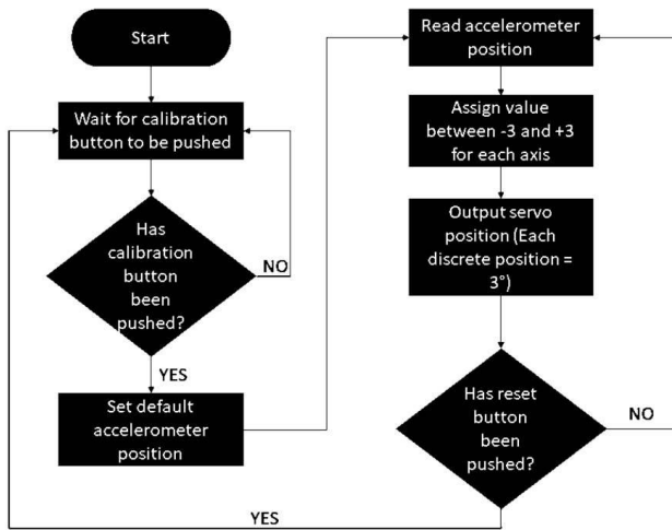
Fig. 8. Flowchart of the joystick manipulator Arduino Program.
