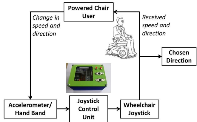
Fig. 7. Operational feedback loop of the joystick manipulator system.
