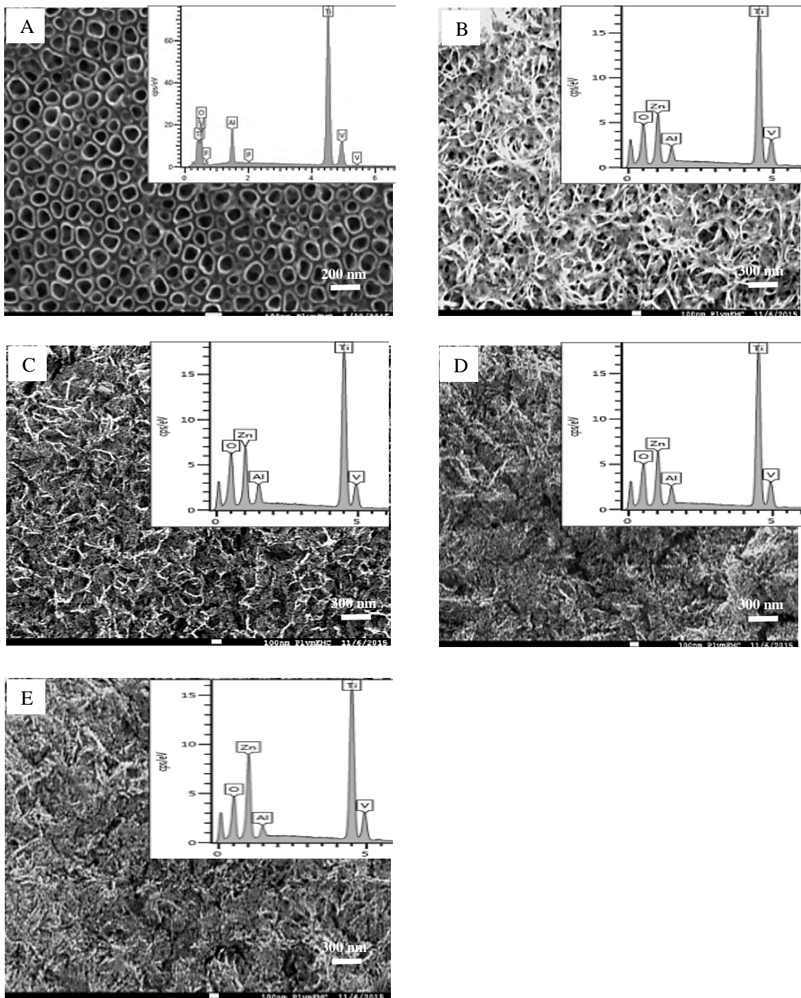
Figure 1: SEM images of Ti alloy surface with (A) the self assembled titania nanotubes ( \text{TiO}_2 NTs), (B) nZnO grown on the \text{TiO}_2 NTs without any heat treatment, and nZnO grown on the \text{TiO}_2 NTs after heating to either, (C) 350 °C, (D) 450 °C, or (E) 550 °C. There was no hydroxyapatite added to these samples. The insert in each panel shows the elemental composition of the coatings by EDS. Images are examples from at least three replicates.
