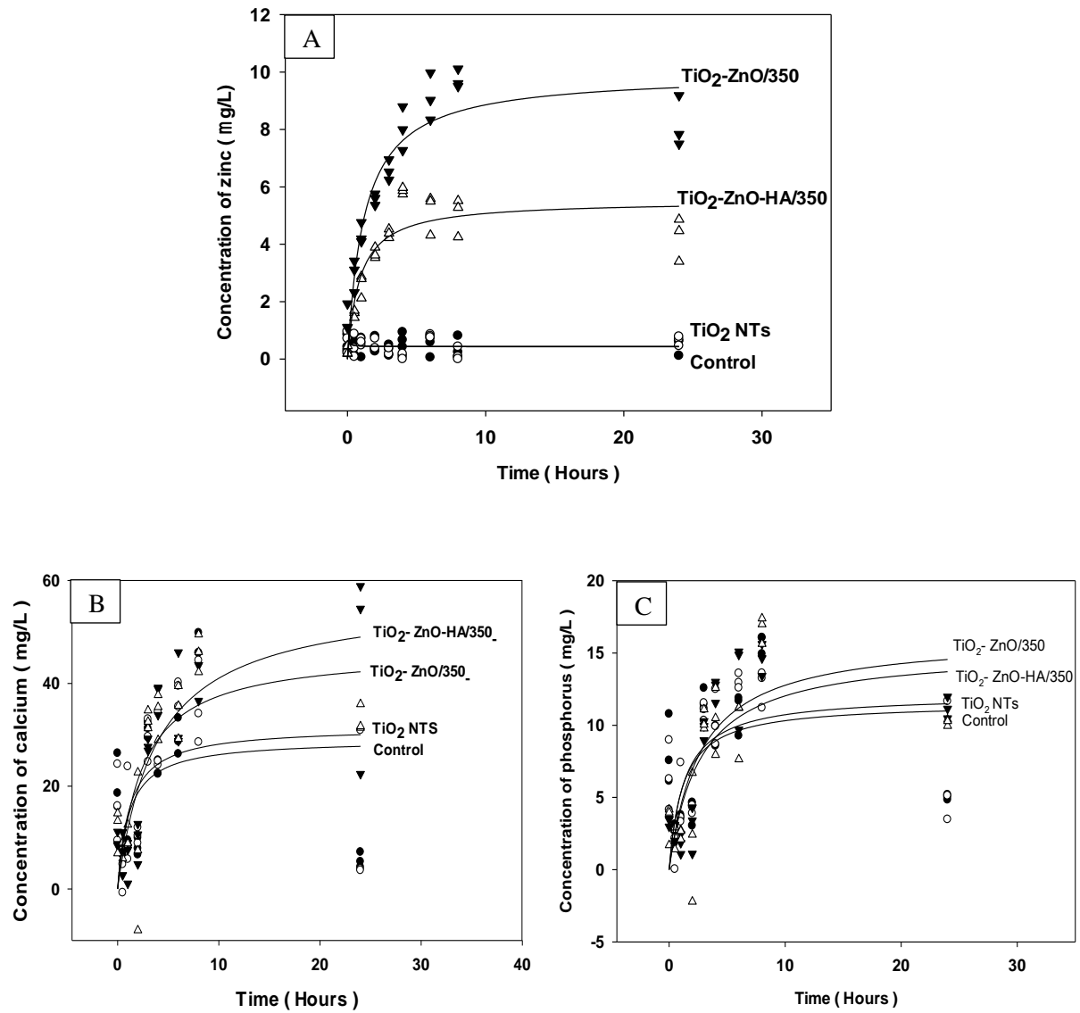
Figure 4: Dialysis of titanium alloy discs coated with either \text{TiO}_2 NTs (• Symbol), \text{TiO}_2 NTs decorated with nZnO ( \text{TiO}_2\text{-ZnO/350} , ▼ Symbol), or also with hydroxyapatite ( \text{TiO}_2\text{-ZnO-HA/350} , Δ Symbol) in simulated body fluid ( 1 \times \text{SBF} ). Concentration of (A) total zinc measured by the ICP-MS, (B) total calcium and (C) total phosphorus measured by the ICP-OES, in SBF from the dialysis in the external compartment of the beakers. Data are single values from triplicate beakers. The curves were fitted to the raw data using a rectangular hyperbola in SigmaPlot.
