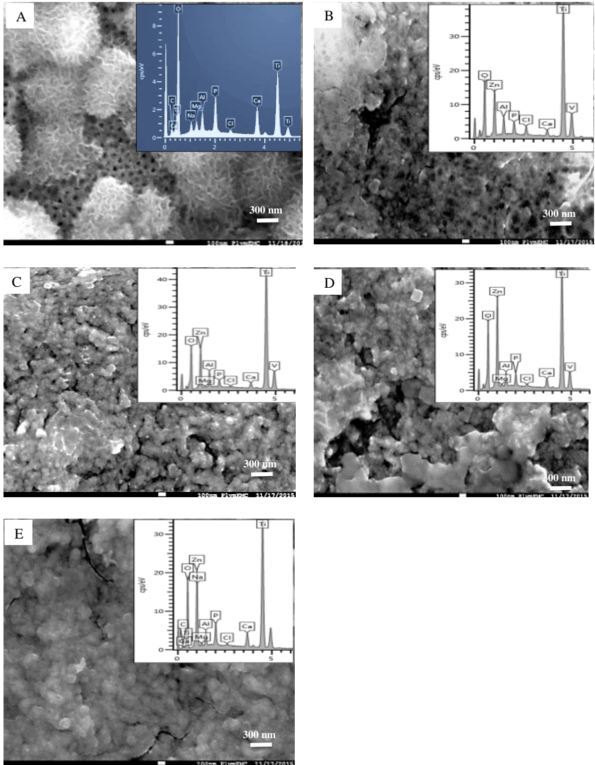
Figure 2: SEM images of HA nanoparticles on top of Ti alloy. (A) The self assembled titania nanotubes (TiO 2 NTs) with hydroxyapatite (HA), (B) nZnO grown on the TiO 2 NTs without any heat treatment, or nZnO grown on the TiO 2 NTs after heating to either, (C) 350 °C, (D) 450 °C, (E) 550 °C. The insert in each panel shows the elemental composition of the coatings by EDS. Images are examples from at least three replicates.
