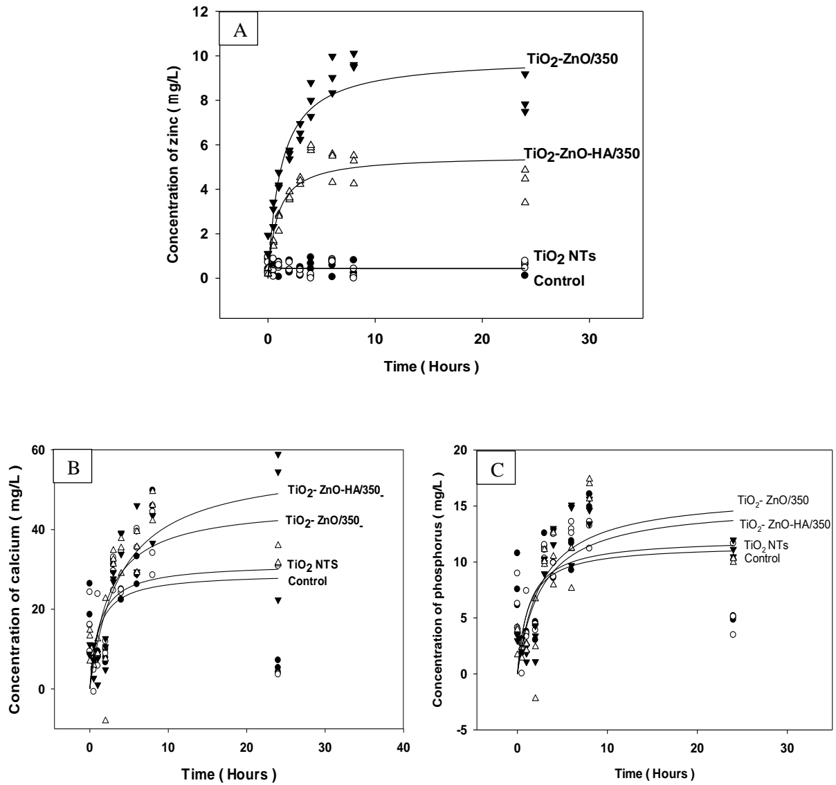
Figure 4: Dialysis of titanium alloy discs coated with either TiO 2 NTs (• Symbol), TiO 2 NTs decorated with nZnO (TiO 2 -ZnO/350, ▼ Symbol), or also with hydroxyapatite (TiO 2 -ZnO-HA/350, Δ Symbol) in simulated body fluid (1 × SBF). Concentration of (A) total zinc measured by the ICP-MS, (B) total calcium and (C) total phosphorus measured by the ICP-OES, in SBF from the dialysis in the external compartment of the beakers. Data are single values from triplicate beakers. The curves were fitted to the raw data using a rectangular hyperbola in SigmaPlot.
