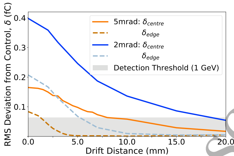
Figure 6. Plot of the values of \delta in the central and edge regions as a function of drift distance for initial beam divergence of 5 mrad (orange lines) and 2 mrad (blue lines). The optimum drift distance occurs when \delta_{edge} falls below the detector threshold of \sim 10 \text{ fC mm}^{-2} . The detector threshold shown is for high-sensitivity image plate as in Ref. [61].
