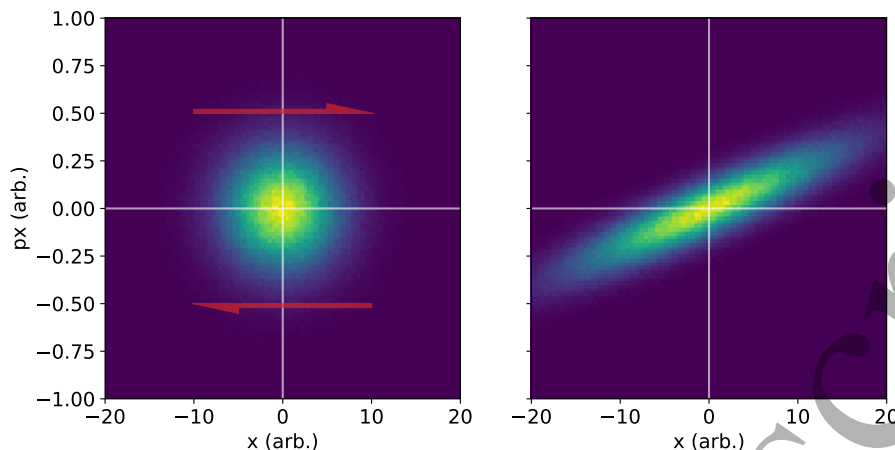
Figure 7. Schematic of x - p_x phase space. The initially uncorrelated electrons (left) become progressively more correlated as they propagate (right).
