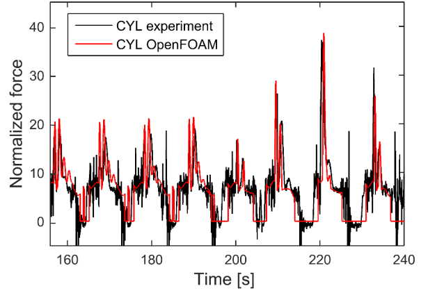
Figure 4: Normalized force. OpenFOAM simulation vs. experiment for the CYL buoy.
