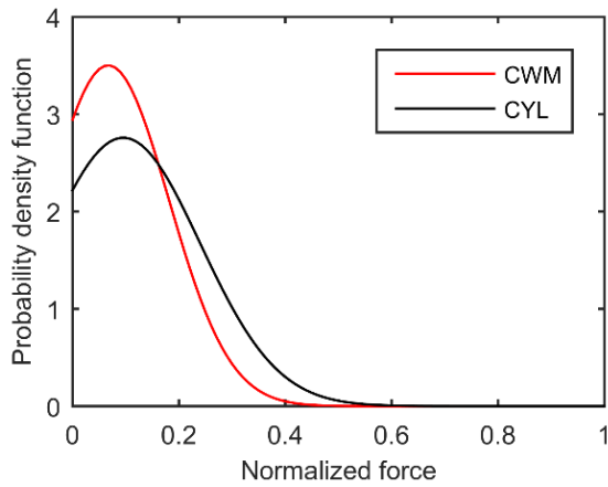
Figure 6: The Gaussian distribution of the line force for the two buoys in irregular waves.
