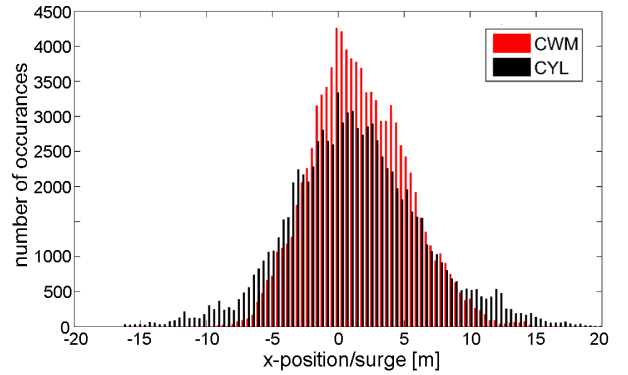
Figure 5: Surge deviation in irregular waves.
