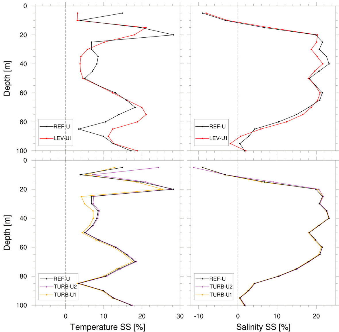
Fig. 17. RMSE skill score for the unstructured grid component of the SURF platform comparing two different vertical stratifications (top panels) and three different vertical turbulence schemes (bottom panels). Temperature (left panels) and salinity (right panels). Skill score is computed considering CTD vertical profiles collected on May 17, 2014. The black line represents the SURF U reference experiment.
