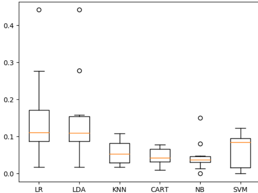
Figure 4: algorithm comparison for location prediction
