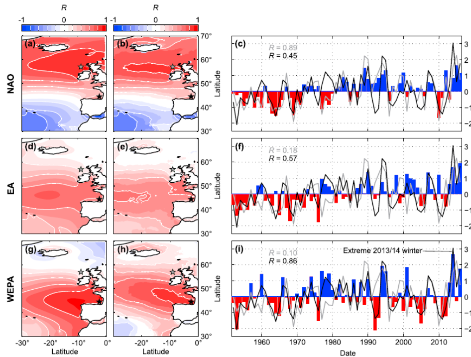
Figure 1.5: (a, b, d, e, g, and h) The spatial correlation of the winter (DJFM)-averaged H_s and H_{s95\%} , respectively, against the winter-averaged NAO (Figures 1.5a and 1.5b) and EA indices (Figures 1.5d and 1.5e), and against our new WEPA index (Figures 1.5g and 1.5h) computed as the normalized SLP difference measured between station Valentia (Ireland) and station Santa Cruz de Tenerife (Canary Islands, Spain). (c, f, and i) Time series of the corresponding indices with superimposed normalized winter-averaged H_s simulated at the buoys SC (Scotland, black) and BI (Biscay, grey) with corresponding correlation coefficient. Source: Castelle et al., 2017 .
