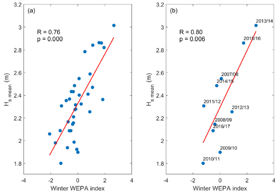
Figure 3.6: Scatter plots of the winter-mean (DJFM) modelled significant wave height, H_{s\ mean} , and the winter WEPA index (a) from the 1980/81 to the 2016/17 winter; and (b) from the 2007/08 to the 2016/17 winter.
