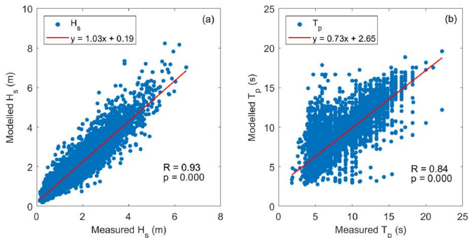
Figure 3.4: Scatter plots of measured and modelled (a) significant wave height, H_s , and (b) peak wave period, T_p , from 2007 to 2017. Measured wave data were obtained from the Perranporth wave buoy (16 m deep) managed by the Channel Coastal Observatory, and 8-km WaveWatch III modelled wave data (50 m deep) were provided by the MetOffice.
