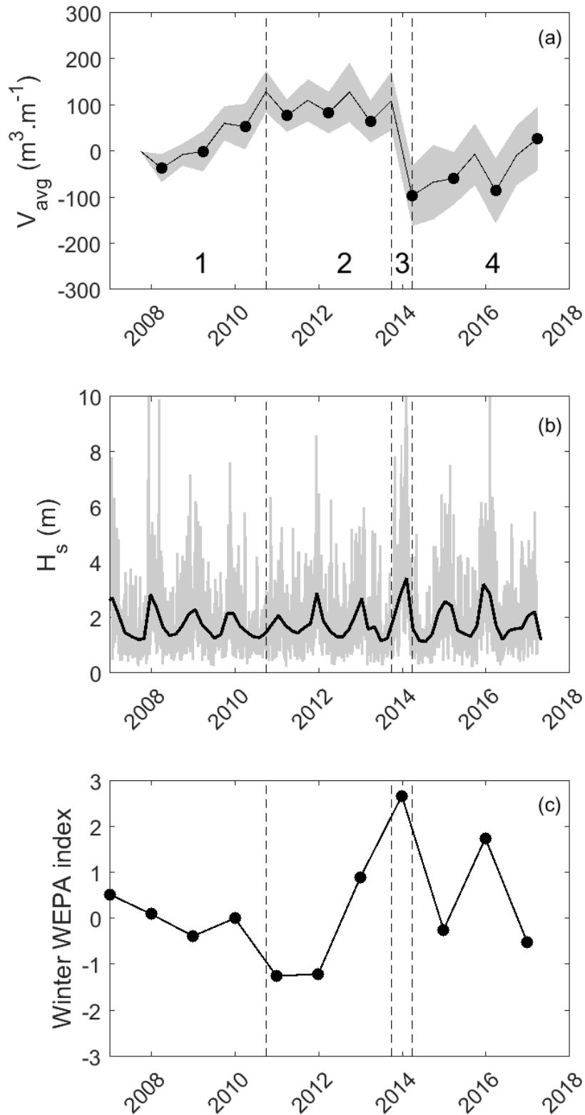
Figure 3.10: Time series from 2007 to 2017 of: (a) the average of the 10 beach volume time-series, V_{avg} ( m^3 \cdot m^{-1} ) in black bounded by its standard deviation in grey; (b) 3-hourly modelled significant wave height H_s (grey) and 8-week block-averaged significant wave height (black); and (c) winter WEPA index. Surveys in spring (end of winter) each year are indicated with black dots to highlight seasonal variations in the beach volume time-series.
