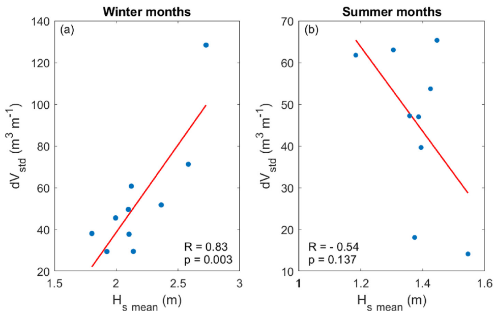
Figure 3.12: Scatter plots of the 10 beaches average standard deviation of 6-monthly volume changes, dV_{std} , and the corresponding 6-monthly significant wave height mean values, H_s mean, over (a) winter months, and (b) summer months from 2007 to 2017.
