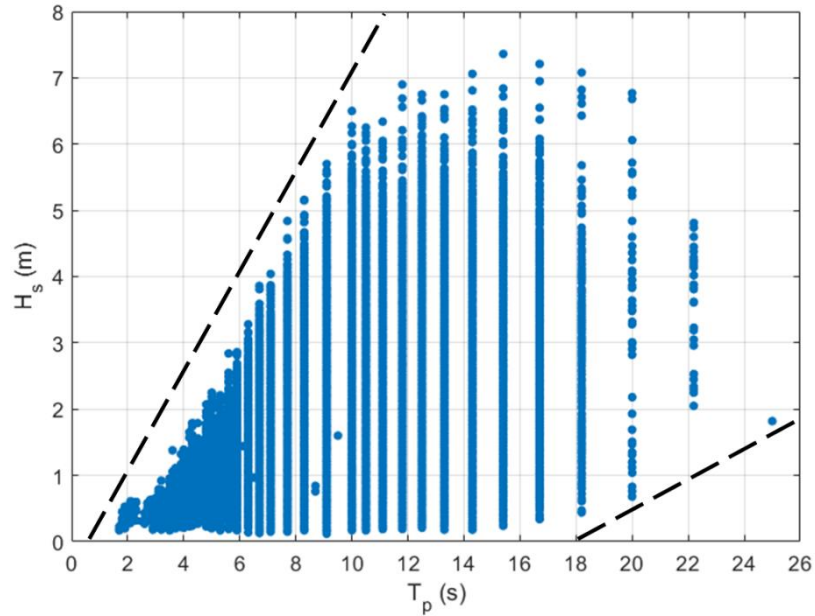
Figure 4.7: Scatter plot of hourly measured significant wave height, H_s , and peak wave period, T_p , recorded by the Perranporth wave buoy from 2007 to 2017. The two dashed lines represent the boundaries of the H_s and T_p values used to force the model.
