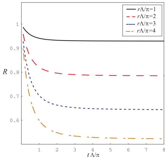
FIG. 1: The ratio R(r, t) defined in (32) for unconfined U(1) . Units are discussed below (33). As the separation of the charges increases the axial state becomes an increasingly poorer description of the ground state.
