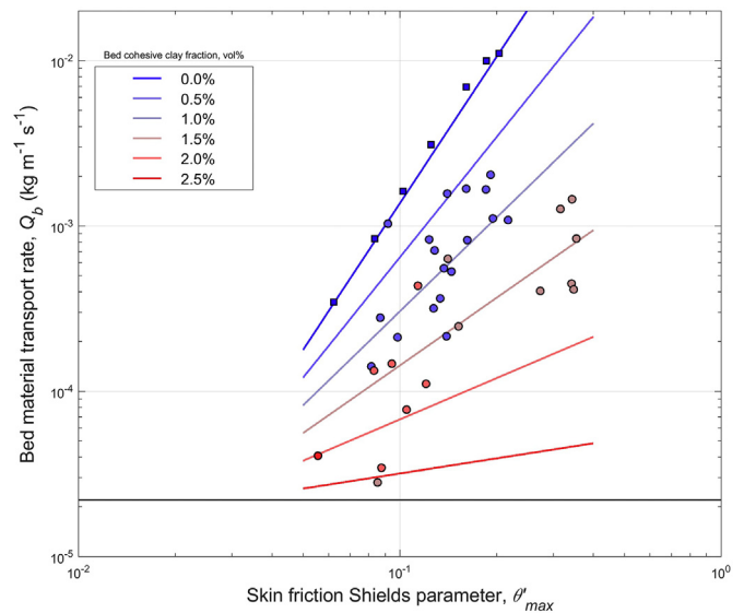
Fig. 11. Maximum bed material transport rate, for flood and ebb, against skin friction Shields parameter for combined currents and waves. The color-filled circles denote the measured data, where the colors represent the bed cohesive clay fraction binned in 0.5 vol% intervals. The black horizontal line represents the minimum bed material transport rate, based on the lowest measurable migration rate by the 3D-ARP and a 0.008 m high bedform (or c = 2.8 vol% in Eq. (11)) and can be treated as the line of no motion. The colored lines denote the multiple linear regression fit, Eq. (11), calculated for set bed cohesive clay content values. The data for clay-free sand ( D_{50} = 238 \mu\text{m} ) from Baas et al. (2000) were included in regression analysis, forcing the fit to these zero cohesive clay fractions (square markers).
