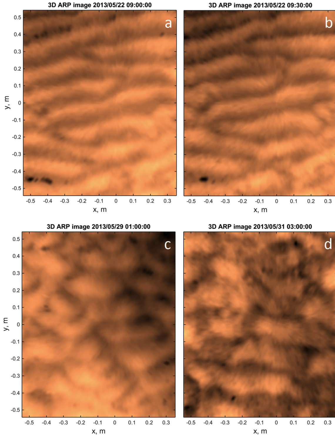
Fig. 8. (a, b) A pair of 3D Acoustic Ripple Profiler (3D-ARP) scans from Site 1. The spatially averaged migration distance, determined by 2D cross-correlation, and migration rate were 0.015\text{ m} and 8.33 \times 10^{-6}\text{ m s}^{-1} , respectively. (c) A 3D-ARP scan from Site 2 showing short-crested, three-dimensional bedforms. (d) A 3D-ARP scan from Site 3 showing two-dimensional sinuous bedforms.
