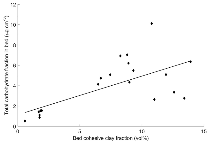
Fig. C1. Total carbohydrate fraction by volume against bed cohesive clay fraction, derived from bed samples collected in the vicinity of Sites 1 to 3 (analyzed for EPS and particle size). The black line represents a robust linear regression fit ( R^2 = 0.42 , p < 0.05 , for n = 20 , total carbohydrate fraction by volume = 0.38c + 1.13 ) between the cohesive clay and total carbohydrate values.
