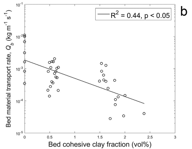
Fig. 10. (a) Relationship between duration of tidal inundation, in hours, and bed cohesive clay content for each tidal inundation period ( n = 27 ). (b) Relationship between bed material transport rate and bed cohesive clay fraction (maximum flood and ebb values for each tidal inundation period, n = 41 ). The data for clay-free sand ( D_{50} = 238 \mu\text{m} ) from Baas et al. (2000) are also included for zero cohesive clay values.
