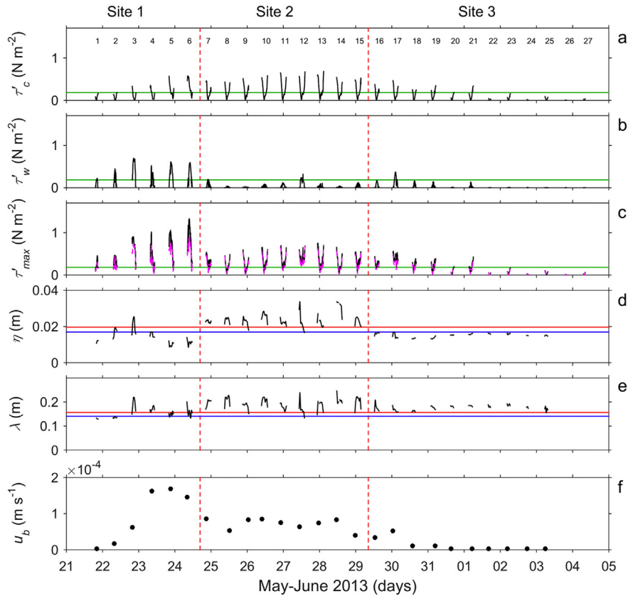
Fig. 7. Time series of (a) current-only bed shear stress, \tau'_c ; (b) wave-only bed shear stress, \tau'_w ; (c) combined maximum bed shear stress, \tau'_{max} and linear maximum bed shear stress, \tau'_{max} (magenta dashed line); (d) bedform height, \eta ; (e) bedform length, \lambda ; and (f) maximum bedform migration rate, u_b , for each tidal cycle derived from the 3D-ARP scans (the rest of the data have been omitted to highlight the overall trend in the record). The vertical red dashed lines mark the times when the instruments were moved between sites. The horizontal green lines denote the critical stress limit of sediment motion from Soulsby and Whitehouse's equation (Soulsby, 1997), for D_{50} = 227 \mu\text{m} , 0.18 \text{ N m}^{-2} . In d and e, the blue and red lines are the equilibrium ripple dimensions of Baas (1999) and Soulsby et al. (2012), respectively. The data shown are for when the tidal flats were inundated with water above the height of the sensors, processed for a 30-min window. The numbers in (a) denote the tidal periods for reference.
