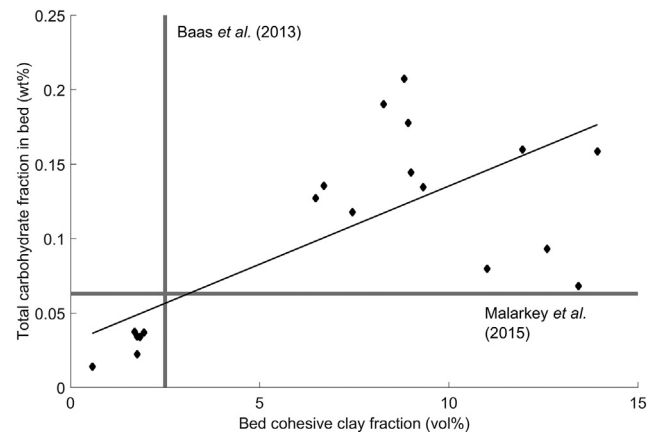
Fig. 5. Total carbohydrate fraction (EPS) against bed cohesive clay fraction, derived from bed samples collected in the vicinity of Sites 1 to 3 (analyzed for EPS and particle size). The thick grey lines represent the thresholds of bedform migration for a bed cohesive clay fraction of 2.5%, based on Baas et al. (2013), and an EPS fraction of 0.063%, based on Malarkey et al. (2015). The values from Site 3 fall to the right of the Baas et al. (2013) line and above the Malarkey et al. (2015) line. The black line represents a robust linear regression fit ( R^2 = 0.41 , p < 0.05 and RMS error = 0.058, for n = 20 , Eq. (10)) between the cohesive clay and EPS values. In appendix C these data are plotted for total carbohydrate per unit volume for comparison with other work (Tolhurst et al., 2005).
