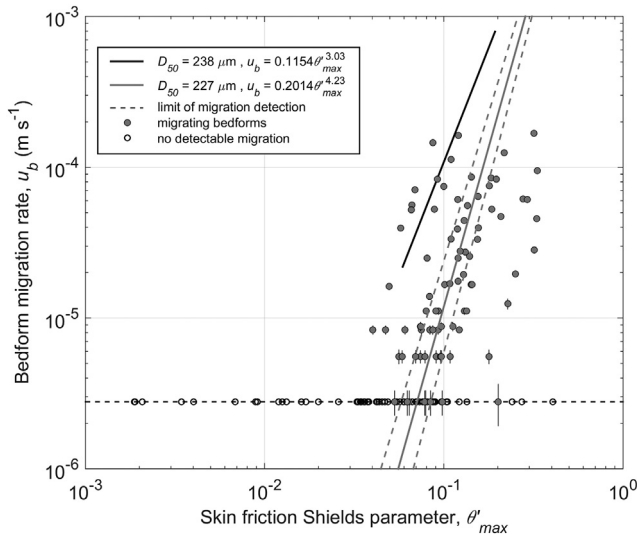
Fig. 9. Bedform migration rate against skin friction Shields parameter for combined currents and waves. The black line denotes the 238 \mu\text{m} regression fit for the clean sand laboratory data of Baas et al. (2000), as in Fig. 1. The dashed black horizontal line and the superimposed open circles denote the lowest measurable migration rates by the 3D-ARP. These data were excluded from the regression analysis. Two extreme values >2.58 standard deviations (outside 99% of the data) were also excluded from the regression analysis. The remaining values were used in the regression fit ( n = 81 ). The regression fit equation for the field data is represented by the solid dark grey line, and the dashed dark grey lines denote the 95% confidence limits of the regression fit line. The error bars for u_b represent the 95% confidence limits of the migration points.
