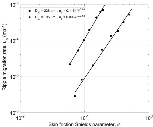
Fig. 1. Empirical relationships between the migration rate of equilibrium current ripples and the skin-friction Shields mobility parameter for two median grain sizes: 238 \mu\text{m} and 95 \mu\text{m} (modified after Baas et al. (2000)). The raw data have been re-processed using the same roughness-length specification of skin friction as for the field data ( z_0 = D_{50} / 12 ).
