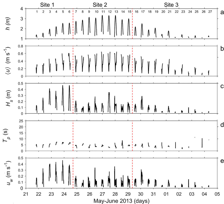
Fig. 6. Time series of (a) water depth, h ; (b) depth-averaged flow velocity (30 min running mean), \langle u \rangle ; (c) significant wave height, H_s ; (d) peak wave period, T_p (smoothed to show trend); and (e) wave bottom orbital amplitude velocity, u_w . The vertical red dashed lines mark the times when the SEDbed frame was moved between sites. The data shown are for when the tidal flats were inundated with water above the height of the sensors, processed for a 30-min window. The wave period data were filtered to show only the wind-generated waves of periods < 25 s (USACE, 2002). The numbers in (a) denote the tidal periods for reference.
