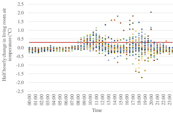
Figure 4 Half hourly indoor air temperature difference on weekends in DW05
