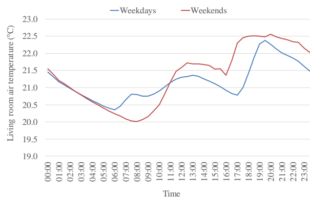
Figure 2 Weekday and weekend living room indoor air temperature profiles in DW05 during the heating season
