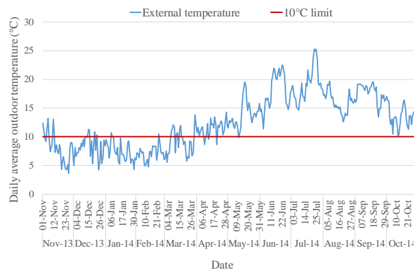
Figure 1 Daily average outdoor air temperatures
