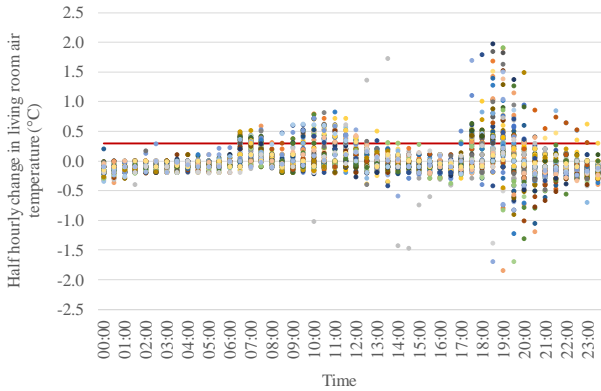
Figure 3 Half hourly indoor air temperature difference on weekdays in DW05
