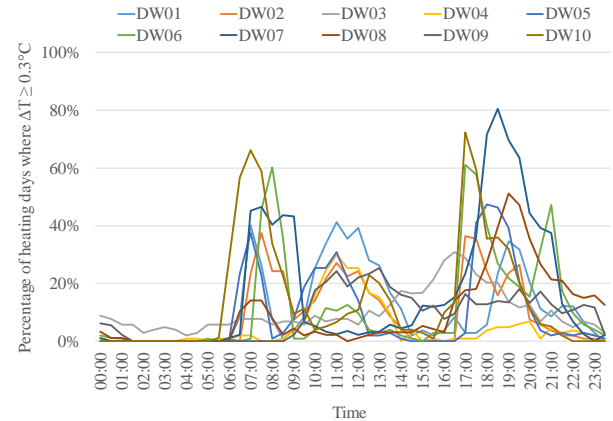
Figure 6 Daily heating profiles on weekday heating days for all case study dwellings
