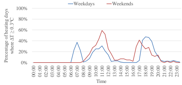
Figure 5 Proportion of heating days for weekdays and weekends during the heating season, where half hourly indoor air temperature increase is at least 0.3^{\circ}\text{C}
