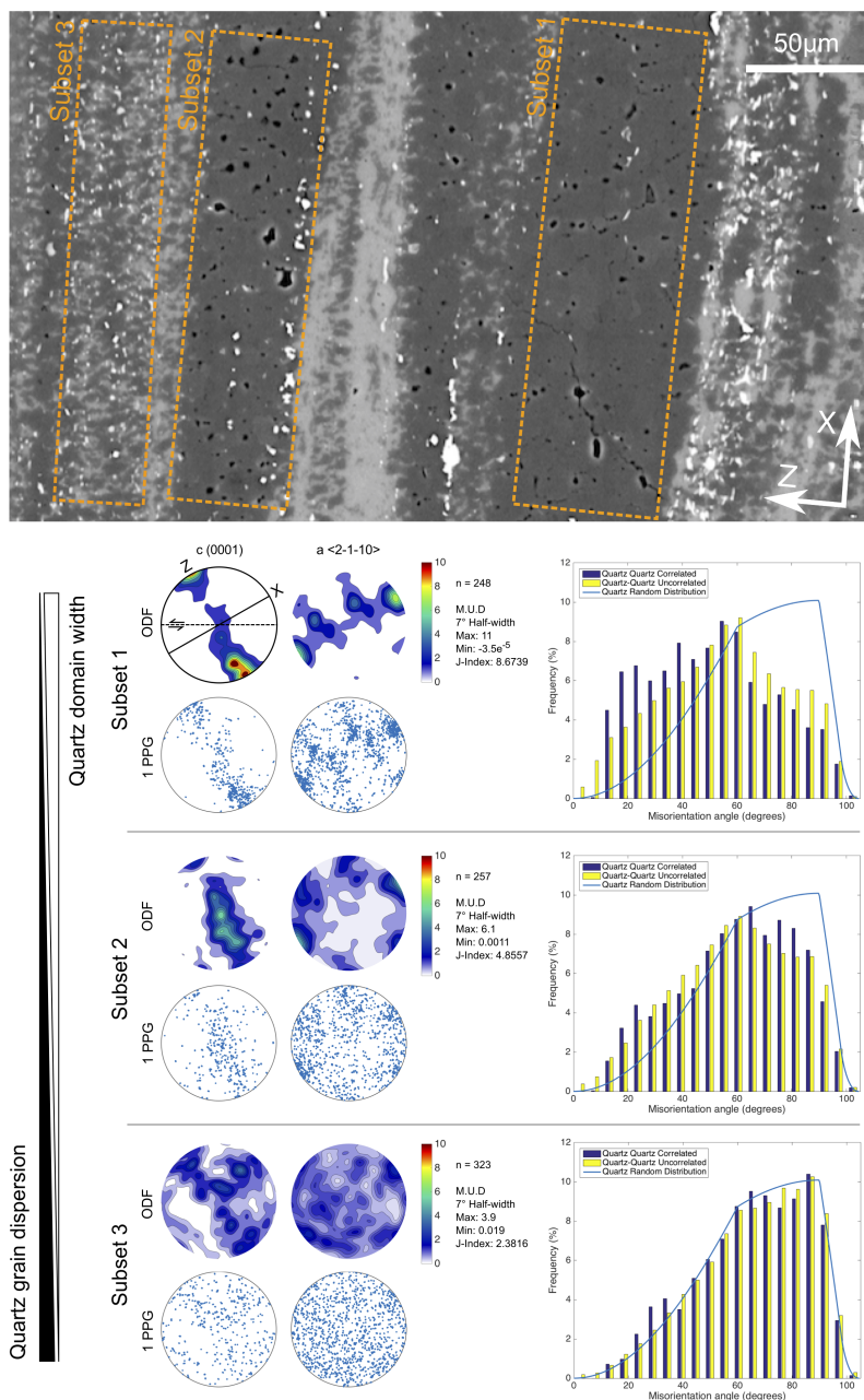
Figure 8. EBSD analyses of quartz domains. The EBSD analyses were performed in the same quartz bands used for subset image analysis (see fig. 1 and 5). EBSD data are presented in equivalent subsets corresponding to decreasing quartz domain width and increasing quartz dispersion. A clear CPO is observed in the pole figure analysis of subset 1 with two c(0001) maxima and two corresponding a<2-1-10> maxima. As quartz domain thickness decreases there is a randomisation of the CPO, highlighted by the decrease in the J-Index and supported by the shift to a near random distribution of the misorientation angle histogram of subset 3.
